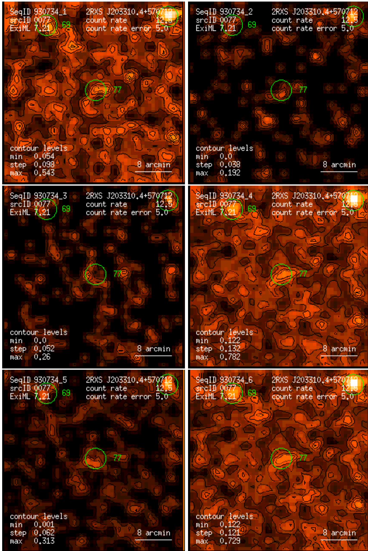
Figure 77: RASS 930734: detection 0077: band rate images, Gaussian filter: (1) PSPC channels 11 – 41, (2) 52 – 90, (3) 91 – 201, (4) 11 – 235, (5) 52 – 201, (6) 11 – 201. Broad band rates in counts/ks. Band rate contour levels in counts/ks/arcmin 2 .
