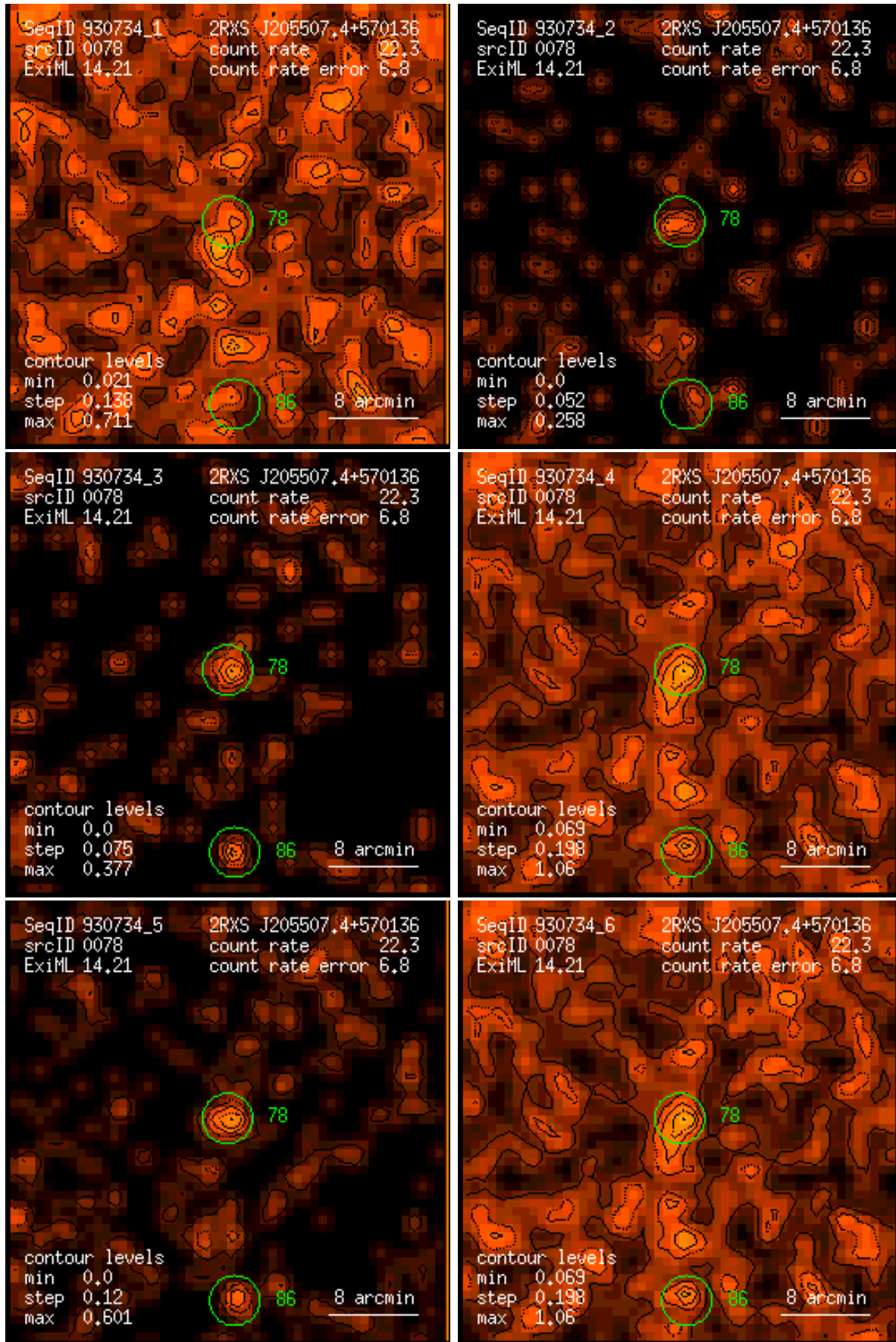
Figure 78: RASS 930734: detection 0078: band rate images, Gaussian filter: (1) PSPC channels 11 – 41, (2) 52 – 90, (3) 91 – 201, (4) 11 – 235, (5) 52 – 201, (6) 11 – 201. Broad band rates in counts/ks. Band rate contour levels in counts/ks/arcmin 2 .
