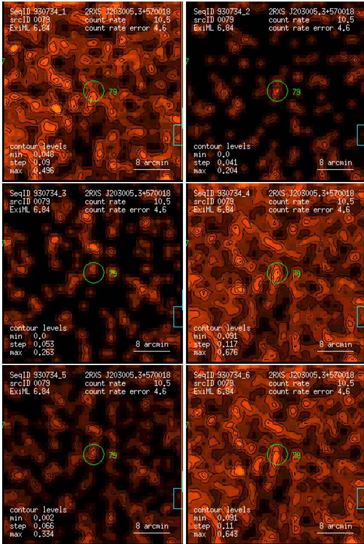
Figure 79: RASS 930734: detection 0079: band rate images, Gaussian filter: (1) PSPC channels 11 – 41, (2) 52 – 90, (3) 91 – 201, (4) 11 – 235, (5) 52 – 201, (6) 11 – 201. Broad band rates in counts/ks. Band rate contour levels in counts/ks/arcmin 2 .
