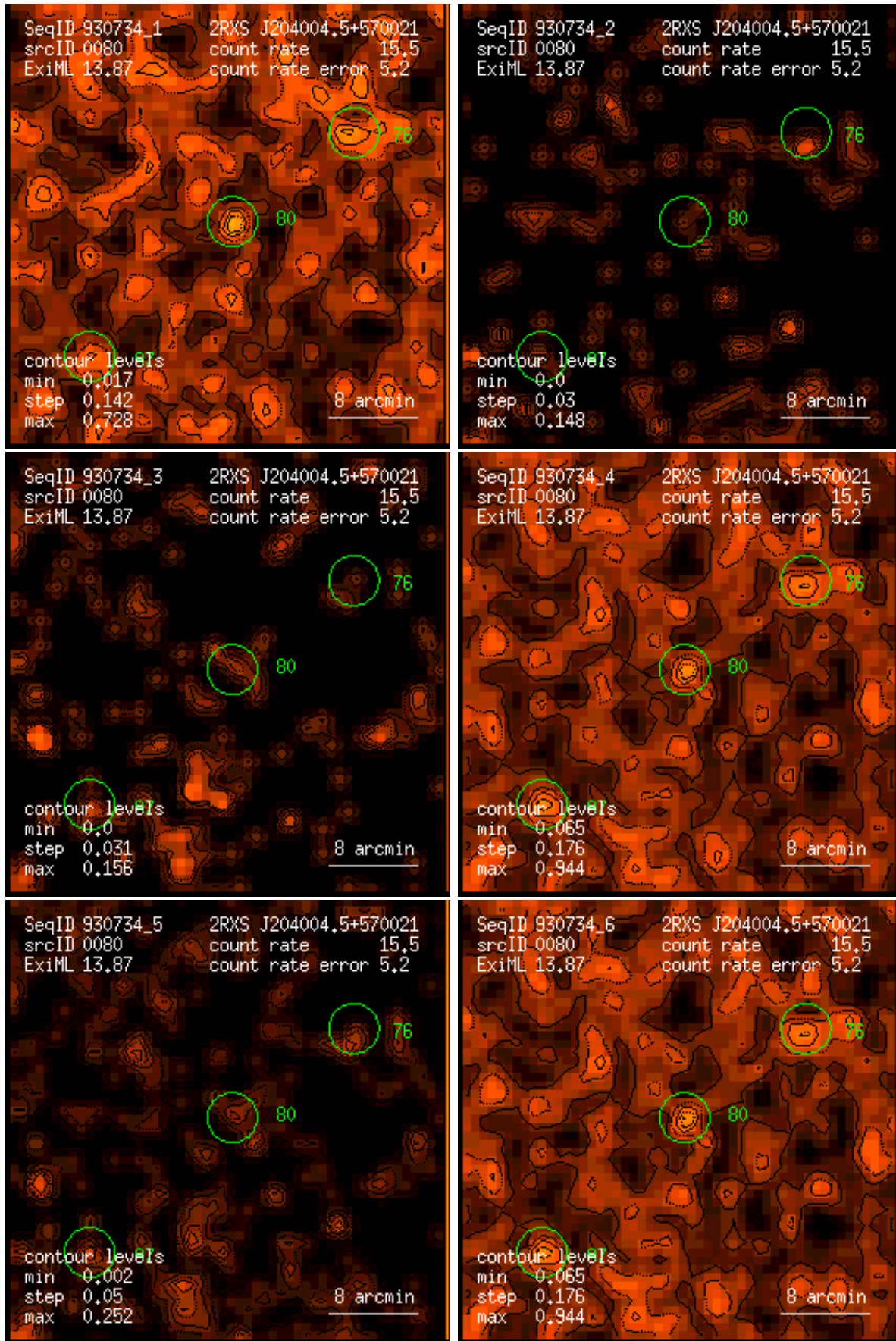
Figure 80: RASS 930734: detection 0080: band rate images, Gaussian filter: (1) PSPC channels 11 – 41, (2) 52 – 90, (3) 91 – 201, (4) 11 – 235, (5) 52 – 201, (6) 11 – 201. Broad band rates in counts/ks. Band rate contour levels in counts/ks/arcmin 2 .
