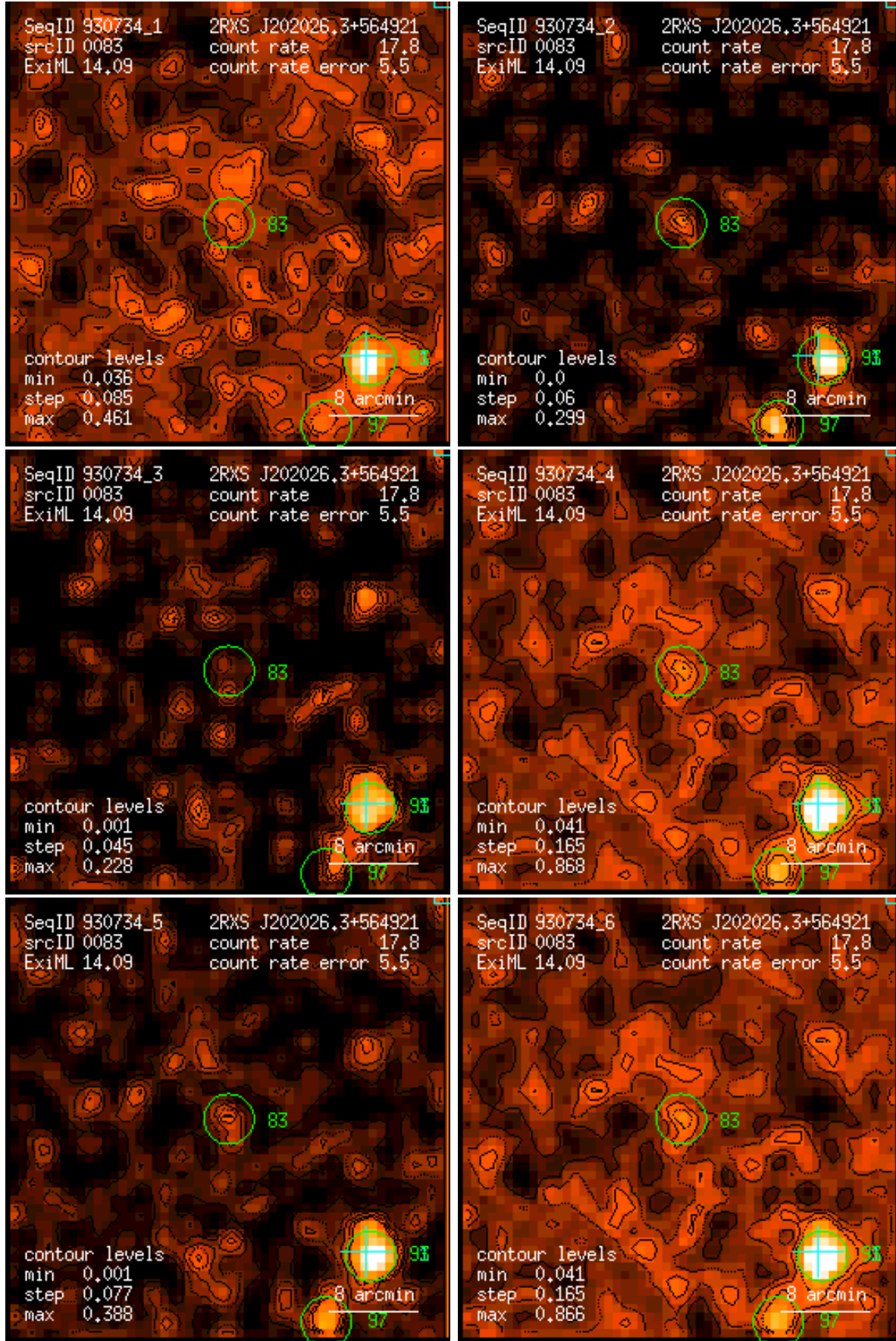
Figure 83: RASS 930734: detection 0083: band rate images, Gaussian filter: (1) PSPC channels 11 – 41, (2) 52 – 90, (3) 91 – 201, (4) 11 – 235, (5) 52 – 201, (6) 11 – 201. Broad band rates in counts/ks. Band rate contour levels in counts/ks/arcmin 2 .
