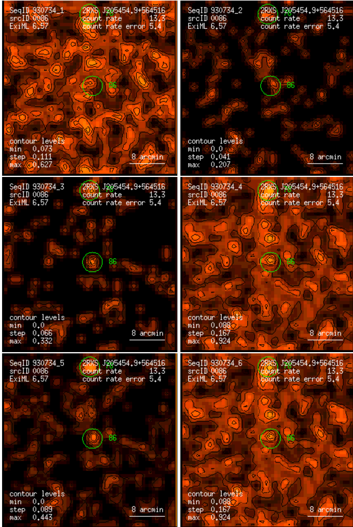
Figure 86: RASS 930734: detection 0086: band rate images, Gaussian filter: (1) PSPC channels 11 – 41, (2) 52 – 90, (3) 91 – 201, (4) 11 – 235, (5) 52 – 201, (6) 11 – 201. Broad band rates in counts/ks. Band rate contour levels in counts/ks/arcmin 2 .
