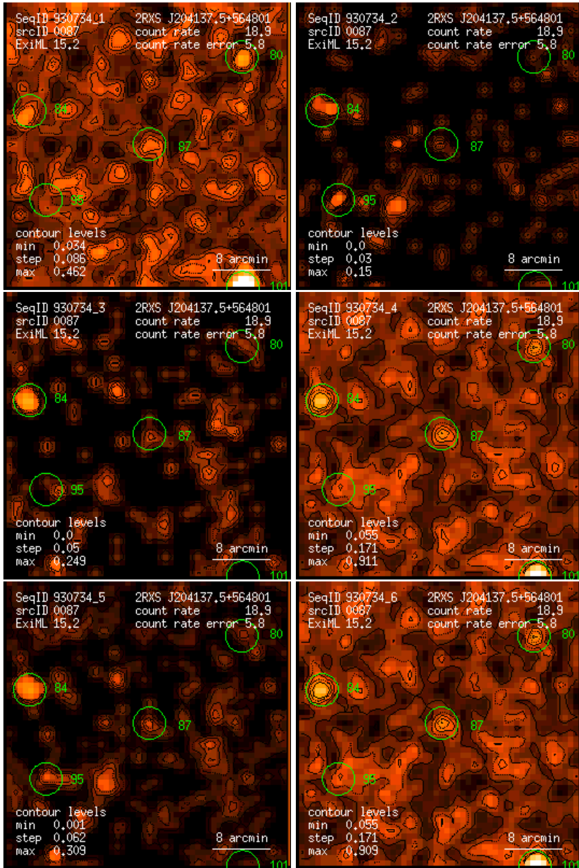
Figure 87: RASS 930734: detection 0087: band rate images, Gaussian filter: (1) PSPC channels 11 – 41, (2) 52 – 90, (3) 91 – 201, (4) 11 – 235, (5) 52 – 201, (6) 11 – 201. Broad band rates in counts/ks. Band rate contour levels in counts/ks/arcmin 2 .
