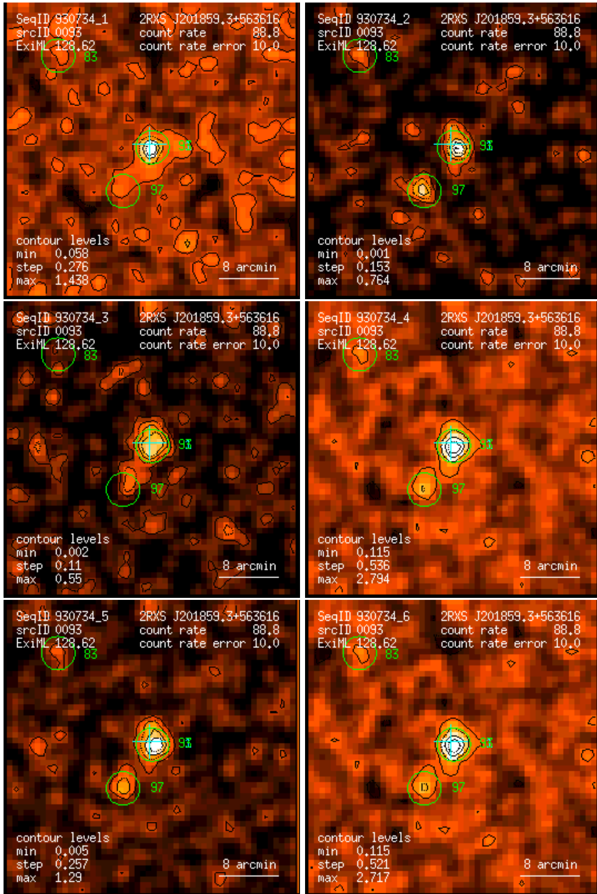
Figure 93: RASS 930734: detection 0093: band rate images, Gaussian filter: (1) PSPC channels 11 – 41, (2) 52 – 90, (3) 91 – 201, (4) 11 – 235, (5) 52 – 201, (6) 11 – 201. Broad band rates in counts/ks. Band rate contour levels in counts/ks/arcmin 2 .
