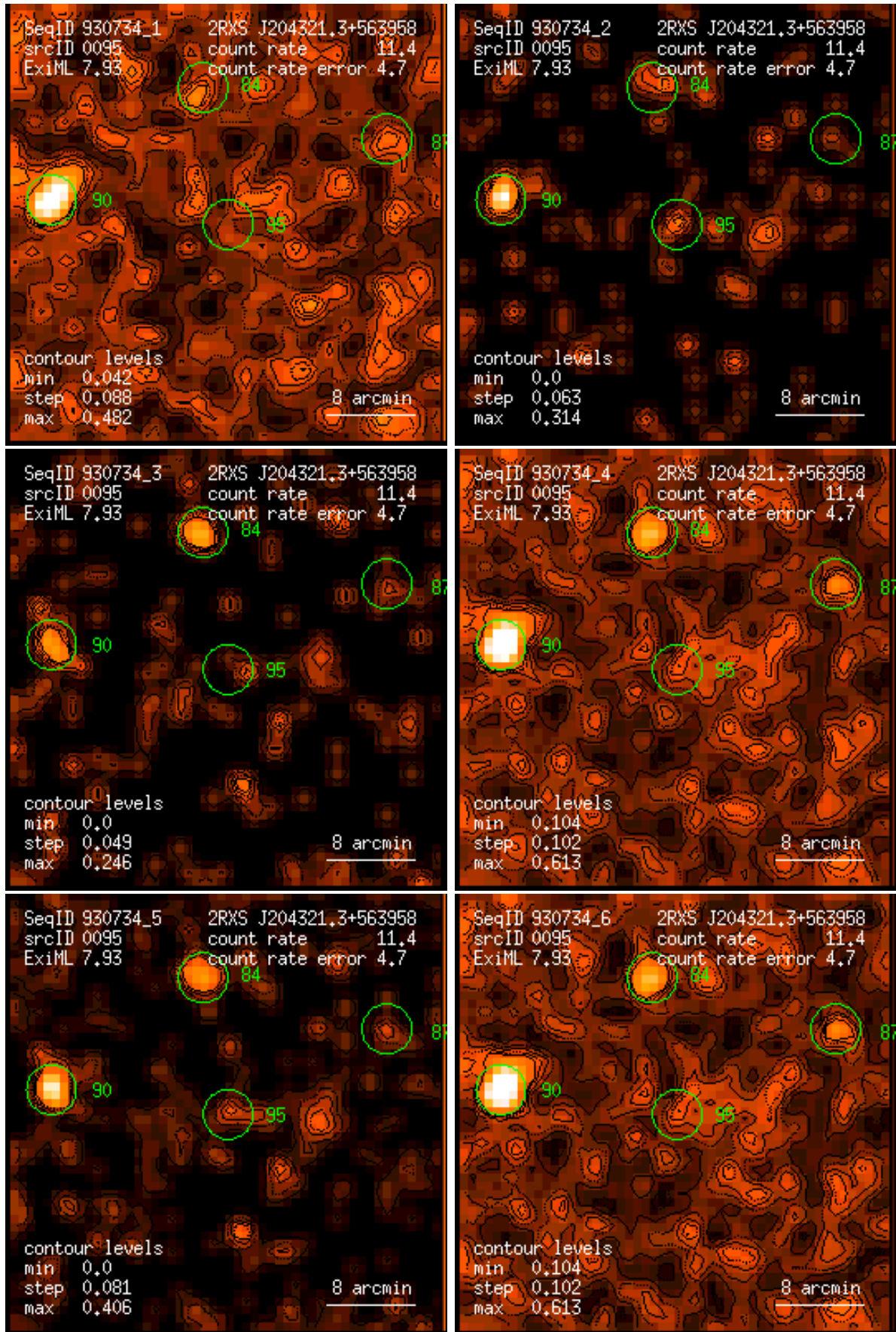
Figure 95: RASS 930734: detection 0095: band rate images, Gaussian filter: (1) PSPC channels 11 – 41, (2) 52 – 90, (3) 91 – 201, (4) 11 – 235, (5) 52 – 201, (6) 11 – 201. Broad band rates in counts/ks. Band rate contour levels in counts/ks/arcmin 2 .
