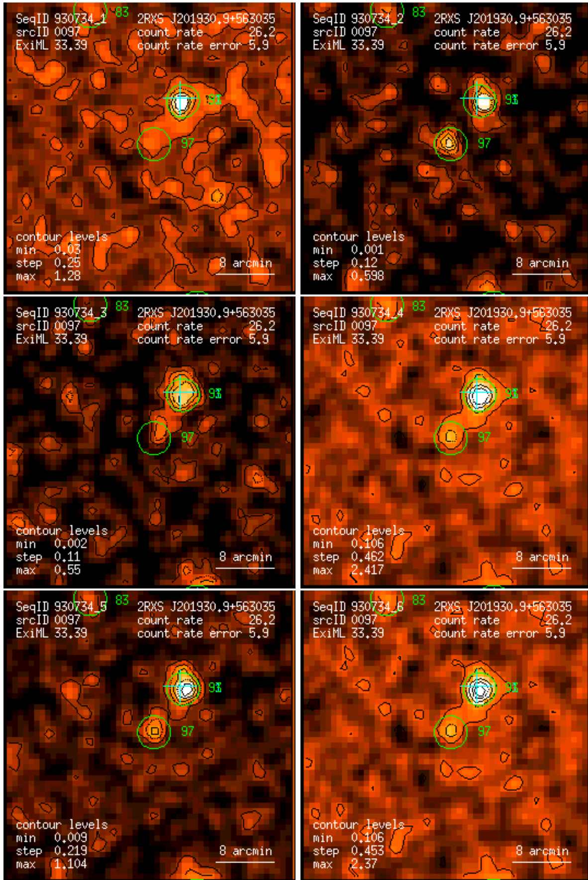
Figure 97: RASS 930734: detection 0097: band rate images, Gaussian filter: (1) PSPC channels 11 – 41, (2) 52 – 90, (3) 91 – 201, (4) 11 – 235, (5) 52 – 201, (6) 11 – 201. Broad band rates in counts/ks. Band rate contour levels in counts/ks/arcmin 2 .
