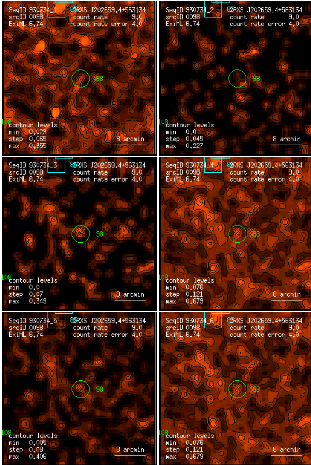
Figure 98: RASS 930734: detection 0098: band rate images, Gaussian filter: (1) PSPC channels 11 – 41, (2) 52 – 90, (3) 91 – 201, (4) 11 – 235, (5) 52 – 201, (6) 11 – 201. Broad band rates in counts/ks. Band rate contour levels in counts/ks/arcmin 2 .
