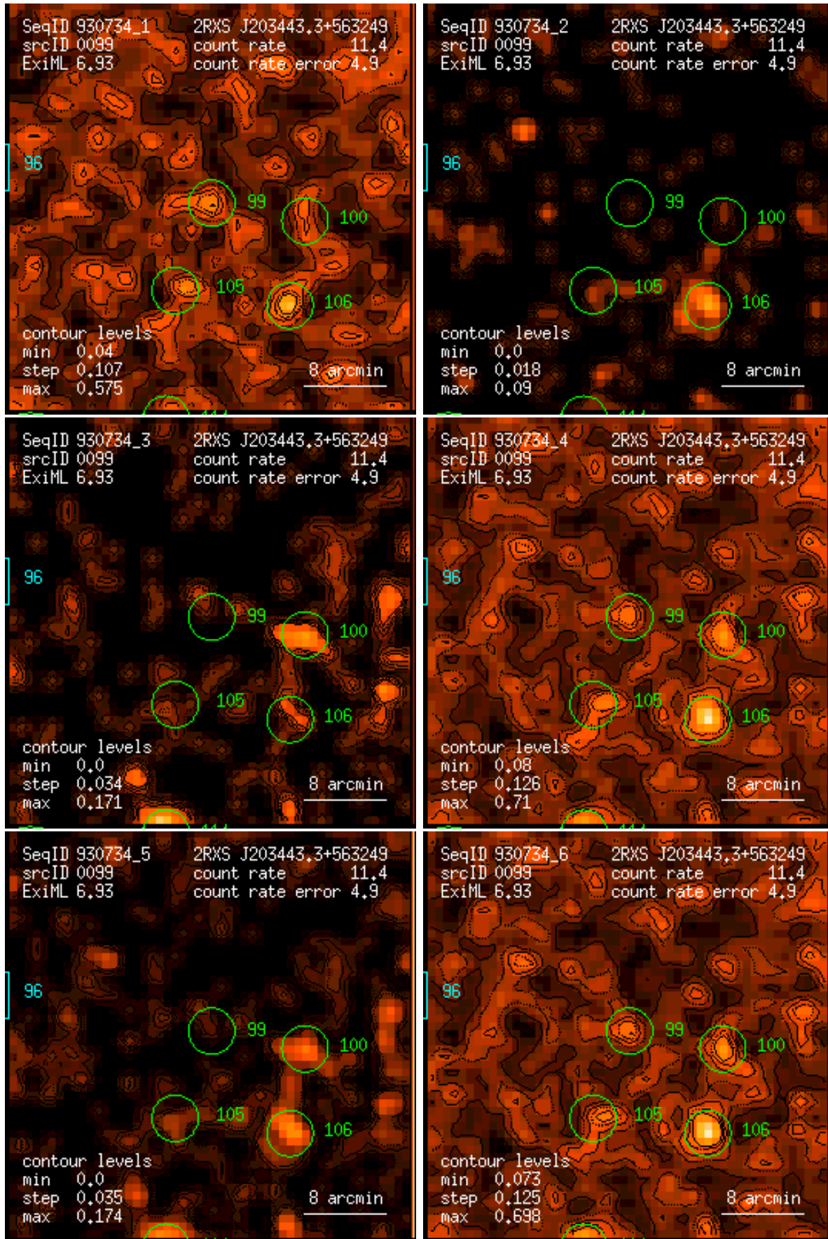
Figure 99: RASS 930734: detection 0099: band rate images, Gaussian filter: (1) PSPC channels 11 – 41, (2) 52 – 90, (3) 91 – 201, (4) 11 – 235, (5) 52 – 201, (6) 11 – 201. Broad band rates in counts/ks. Band rate contour levels in counts/ks/arcmin 2 .
