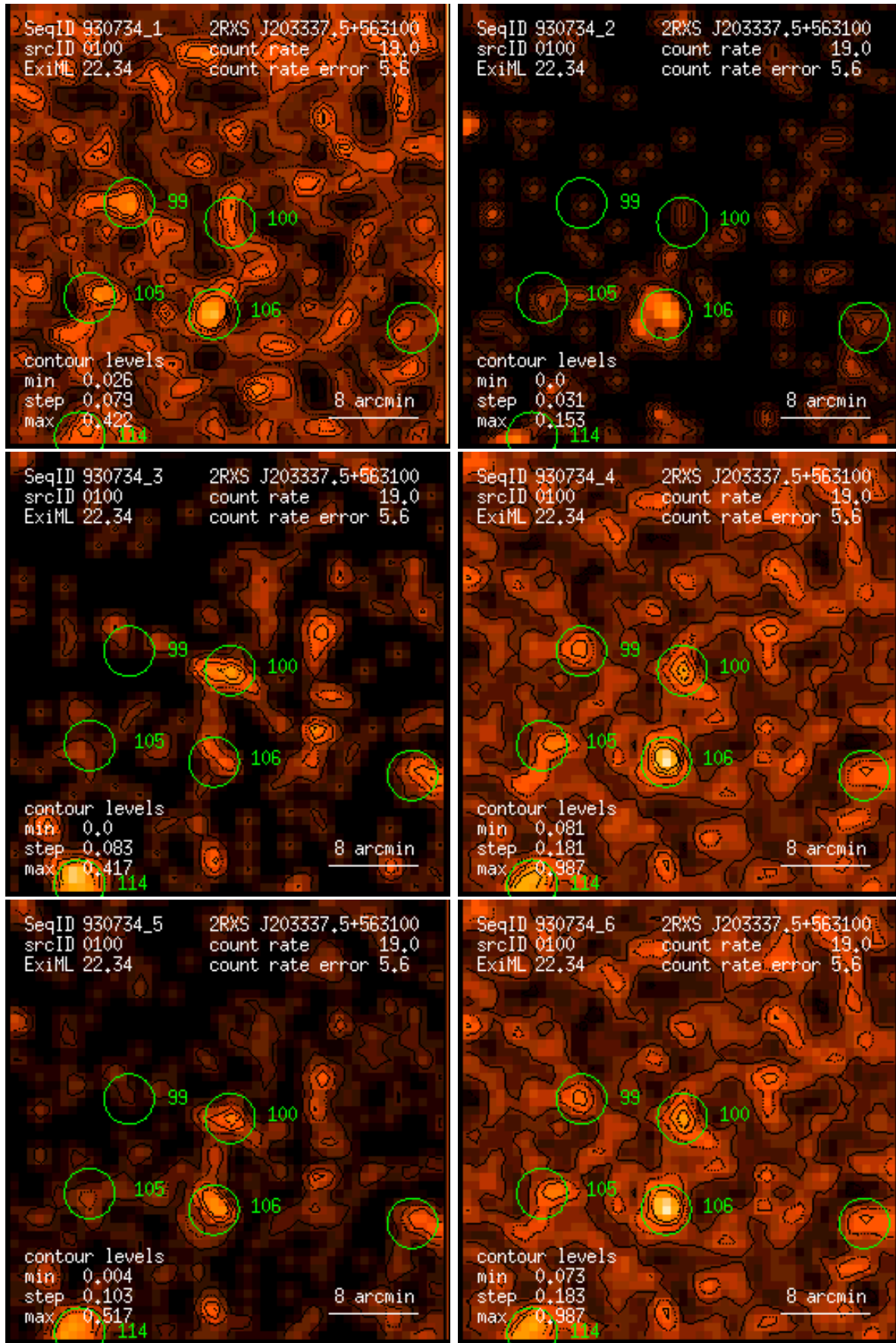
Figure 100: RASS 930734: detection 0100: band rate images, Gaussian filter: (1) PSPC channels 11 – 41, (2) 52 – 90, (3) 91 – 201, (4) 11 – 235, (5) 52 – 201, (6) 11 – 201. Broad band rates in counts/ks. Band rate contour levels in counts/ks/arcmin 2 .
