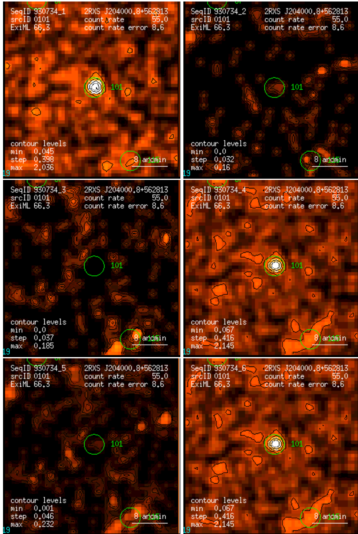
Figure 101: RASS 930734: detection 0101: band rate images, Gaussian filter: (1) PSPC channels 11 – 41, (2) 52 – 90, (3) 91 – 201, (4) 11 – 235, (5) 52 – 201, (6) 11 – 201. Broad band rates in counts/ks. Band rate contour levels in counts/ks/arcmin 2 .
