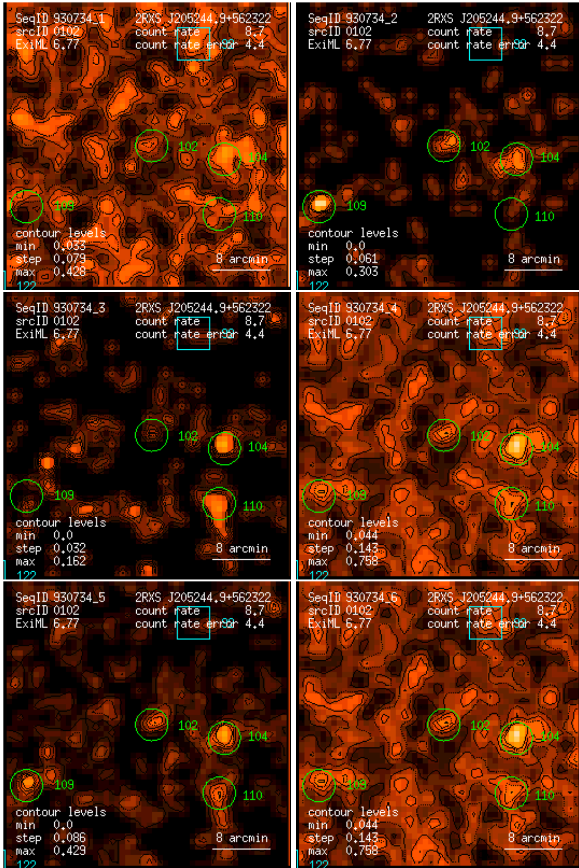
Figure 102: RASS 930734: detection 0102: band rate images, Gaussian filter: (1) PSPC channels 11 – 41, (2) 52 – 90, (3) 91 – 201, (4) 11 – 235, (5) 52 – 201, (6) 11 – 201. Broad band rates in counts/ks. Band rate contour levels in counts/ks/arcmin 2 .
