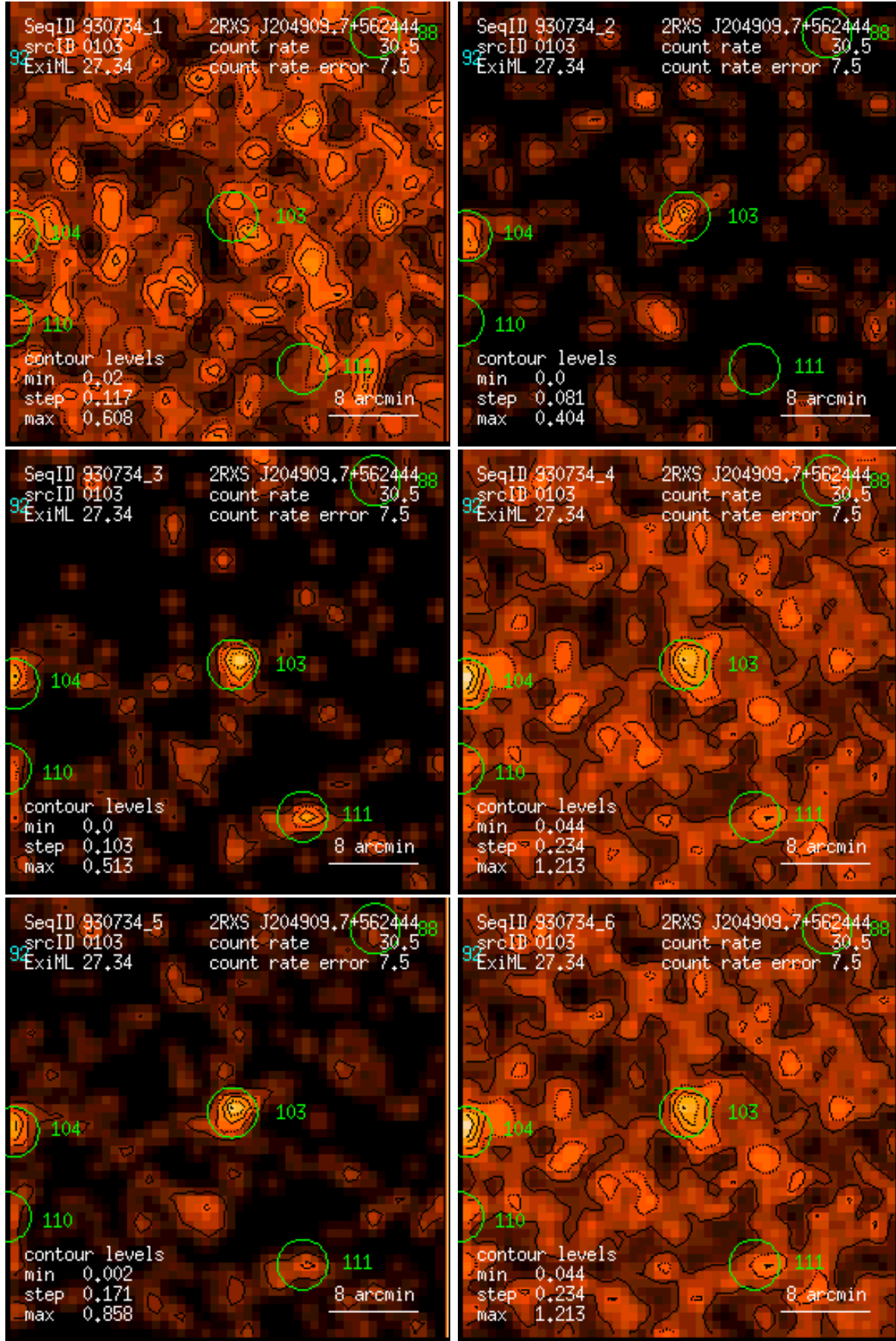
Figure 103: RASS 930734: detection 0103: band rate images, Gaussian filter: (1) PSPC channels 11 – 41, (2) 52 – 90, (3) 91 – 201, (4) 11 – 235, (5) 52 – 201, (6) 11 – 201. Broad band rates in counts/ks. Band rate contour levels in counts/ks/arcmin 2 .
