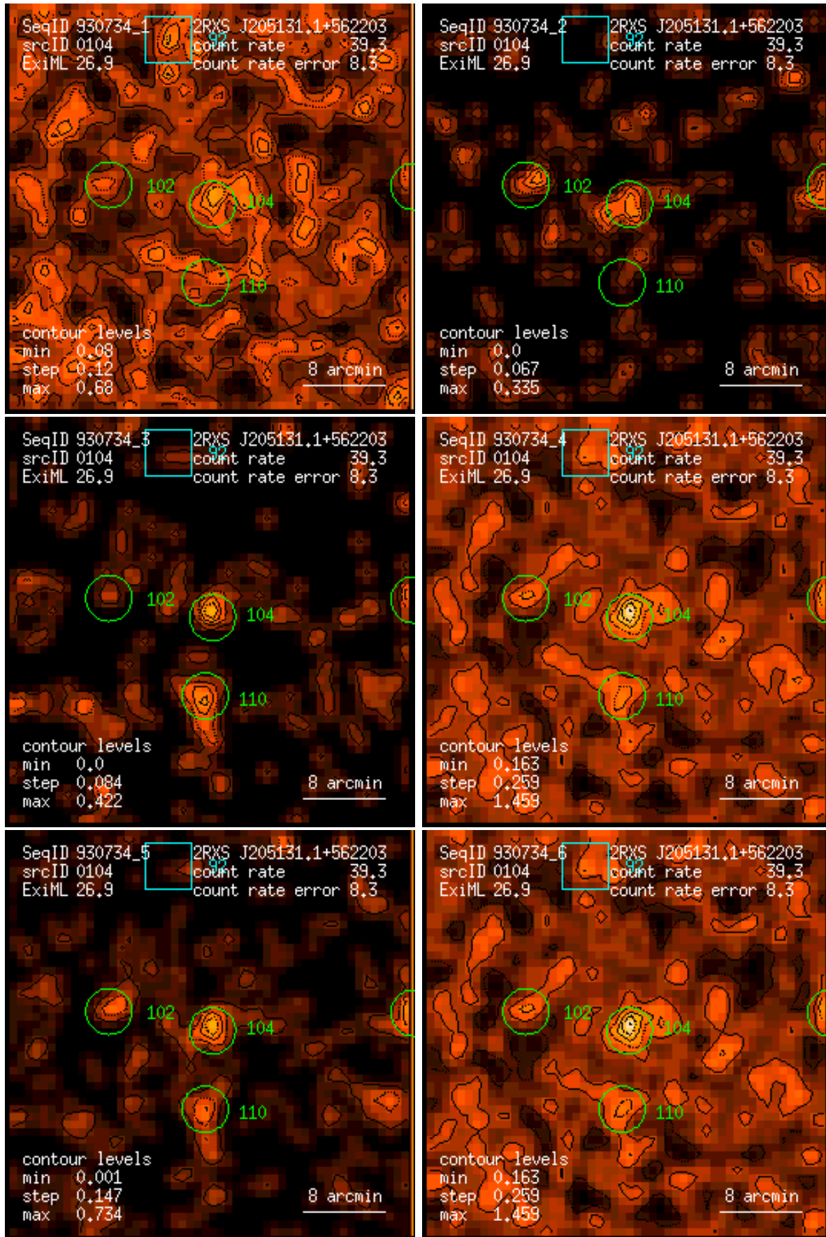
Figure 104: RASS 930734: detection 0104: band rate images, Gaussian filter: (1) PSPC channels 11 – 41, (2) 52 – 90, (3) 91 – 201, (4) 11 – 235, (5) 52 – 201, (6) 11 – 201. Broad band rates in counts/ks. Band rate contour levels in counts/ks/arcmin 2 .
