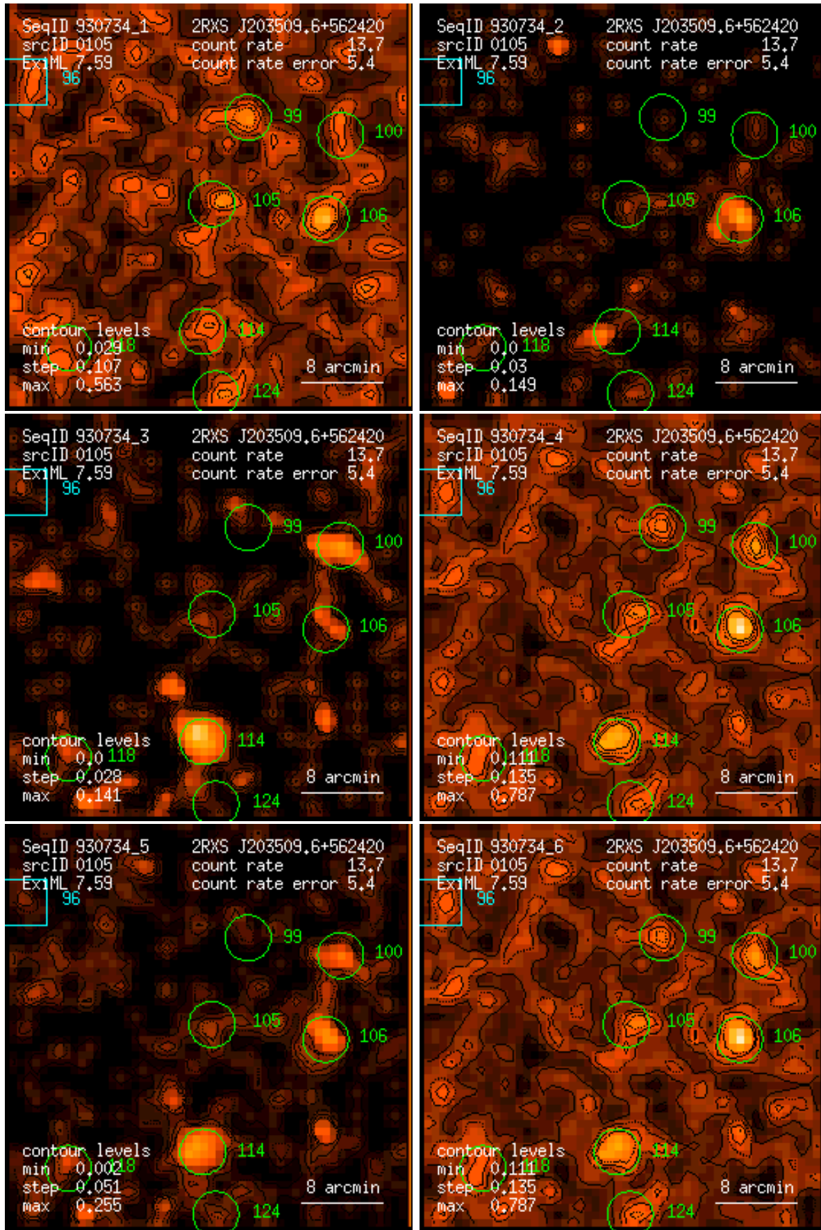
Figure 105: RASS 930734: detection 0105: band rate images, Gaussian filter: (1) PSPC channels 11 – 41, (2) 52 – 90, (3) 91 – 201, (4) 11 – 235, (5) 52 – 201, (6) 11 – 201. Broad band rates in counts/ks. Band rate contour levels in counts/ks/arcmin 2 .
