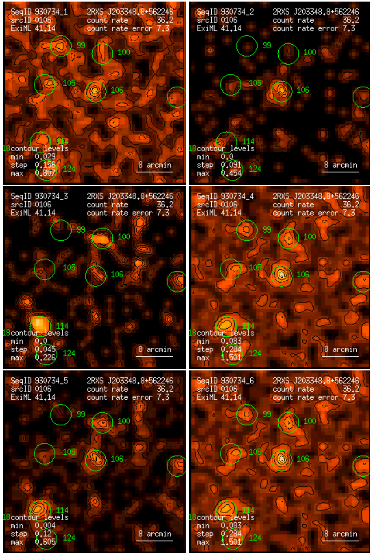
Figure 106: RASS 930734: detection 0106: band rate images, Gaussian filter: (1) PSPC channels 11 – 41, (2) 52 – 90, (3) 91 – 201, (4) 11 – 235, (5) 52 – 201, (6) 11 – 201. Broad band rates in counts/ks. Band rate contour levels in counts/ks/arcmin 2 .
