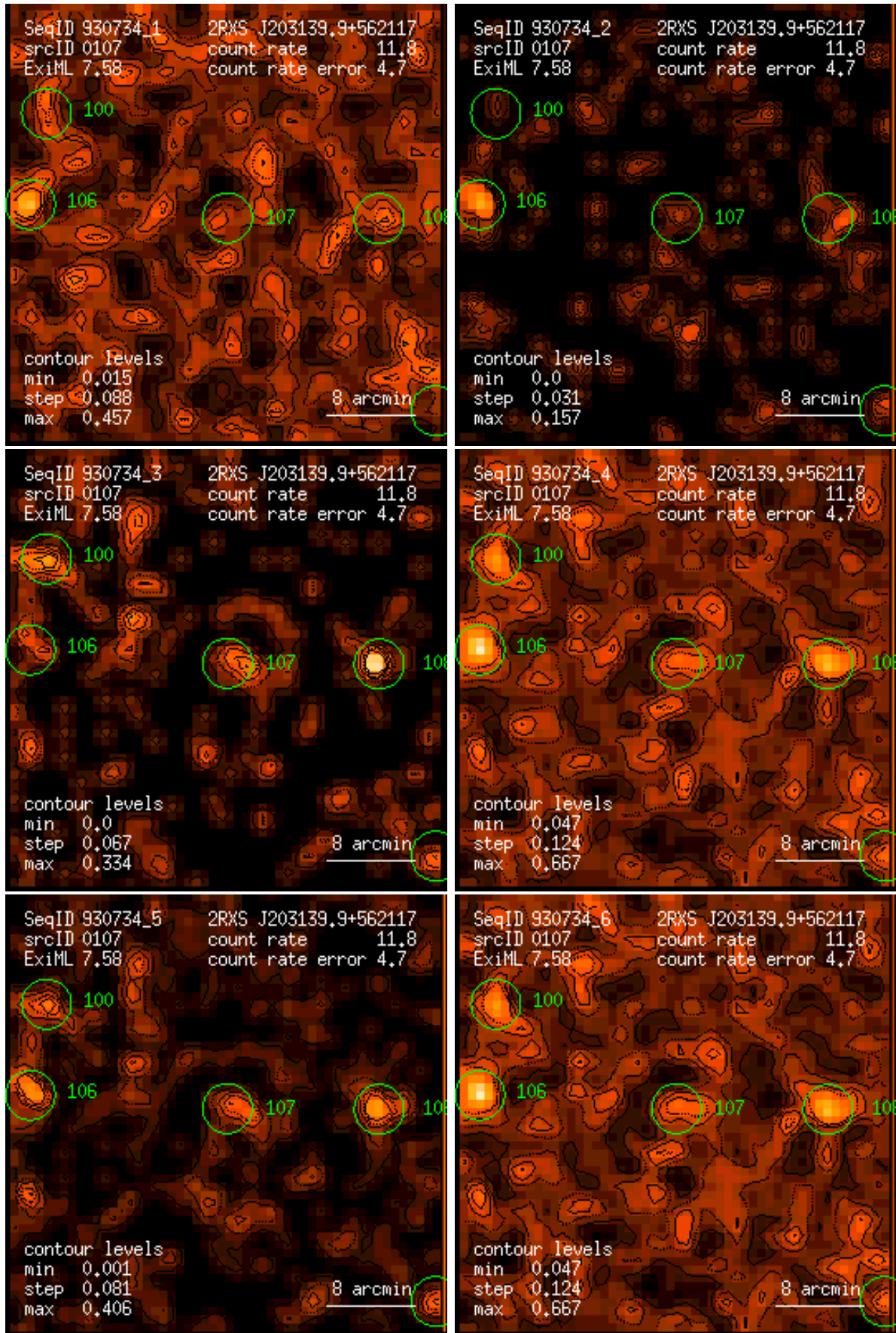
Figure 107: RASS 930734: detection 0107: band rate images, Gaussian filter: (1) PSPC channels 11 – 41, (2) 52 – 90, (3) 91 – 201, (4) 11 – 235, (5) 52 – 201, (6) 11 – 201. Broad band rates in counts/ks. Band rate contour levels in counts/ks/arcmin 2 .
