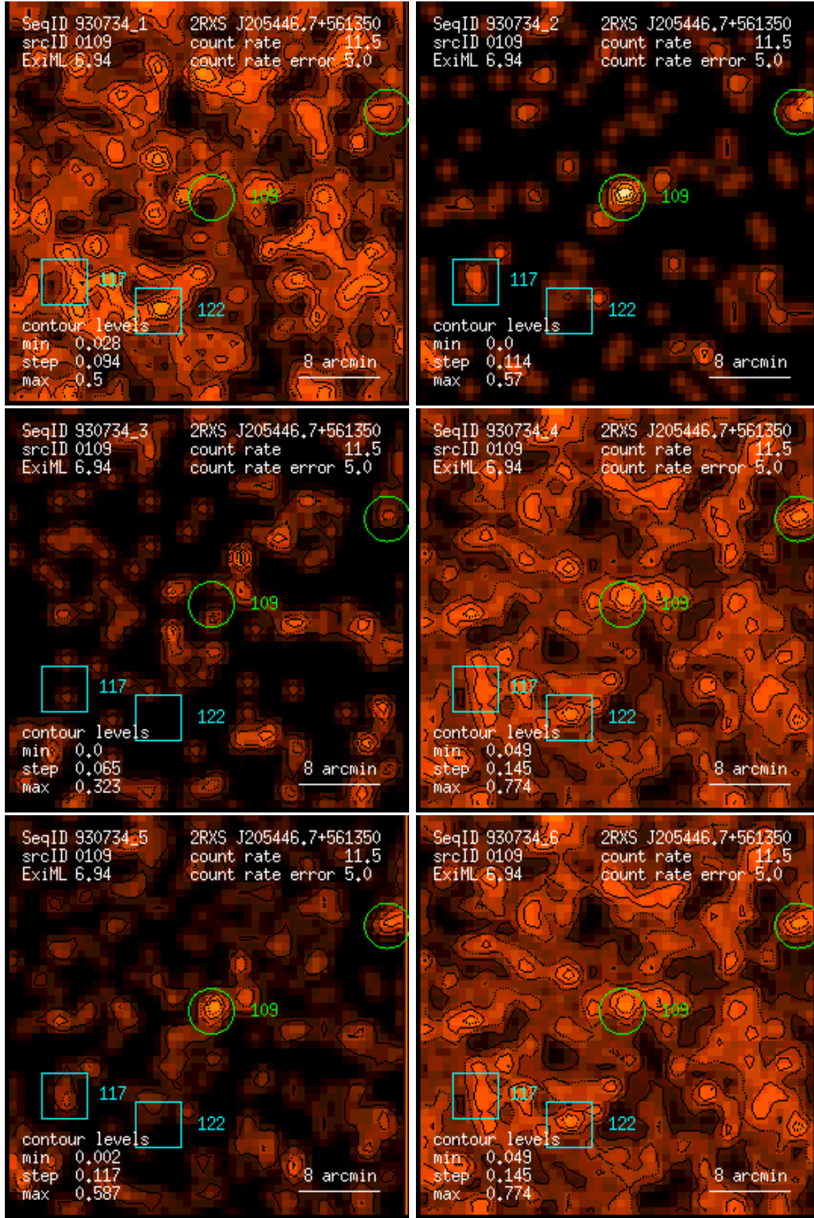
Figure 109: RASS 930734: detection 0109: band rate images, Gaussian filter: (1) PSPC channels 11 – 41, (2) 52 – 90, (3) 91 – 201, (4) 11 – 235, (5) 52 – 201, (6) 11 – 201. Broad band rates in counts/ks. Band rate contour levels in counts/ks/arcmin 2 .
