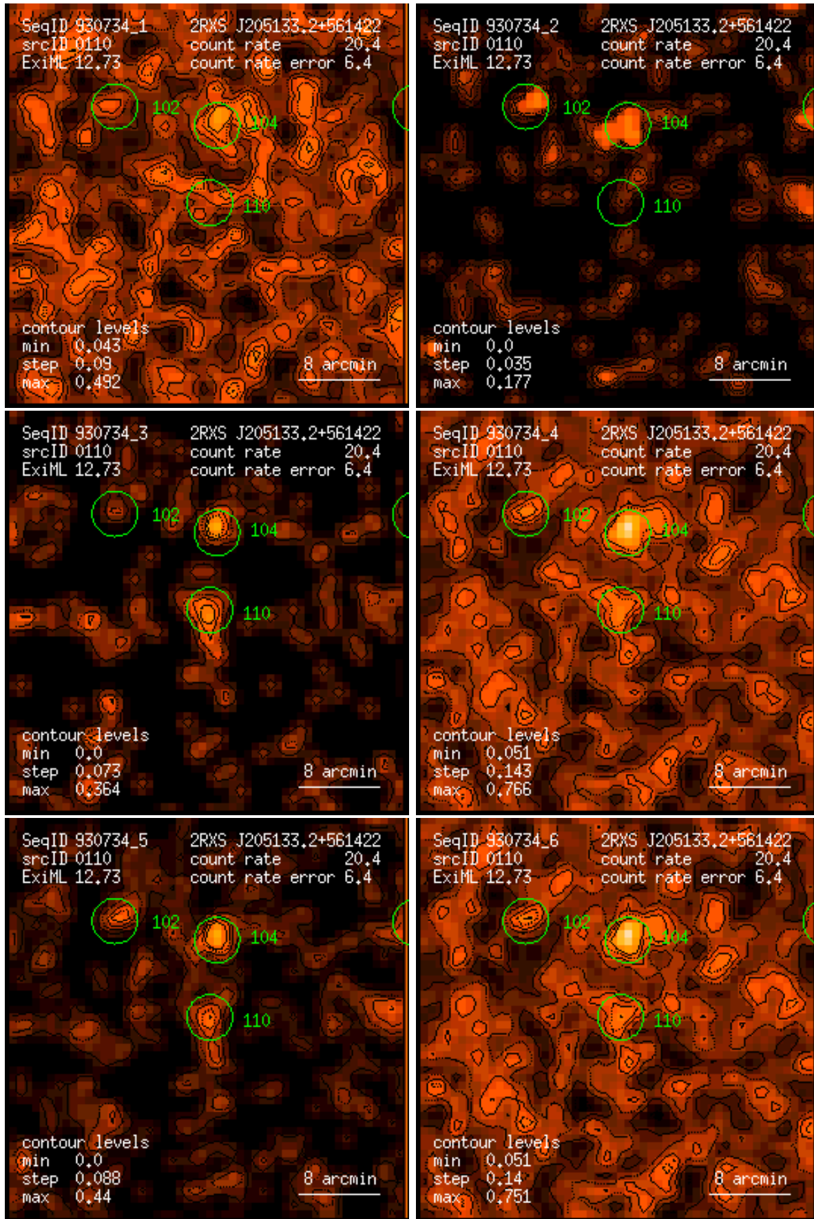
Figure 110: RASS 930734: detection 0110: band rate images, Gaussian filter: (1) PSPC channels 11 – 41, (2) 52 – 90, (3) 91 – 201, (4) 11 – 235, (5) 52 – 201, (6) 11 – 201. Broad band rates in counts/ks. Band rate contour levels in counts/ks/arcmin 2 .
