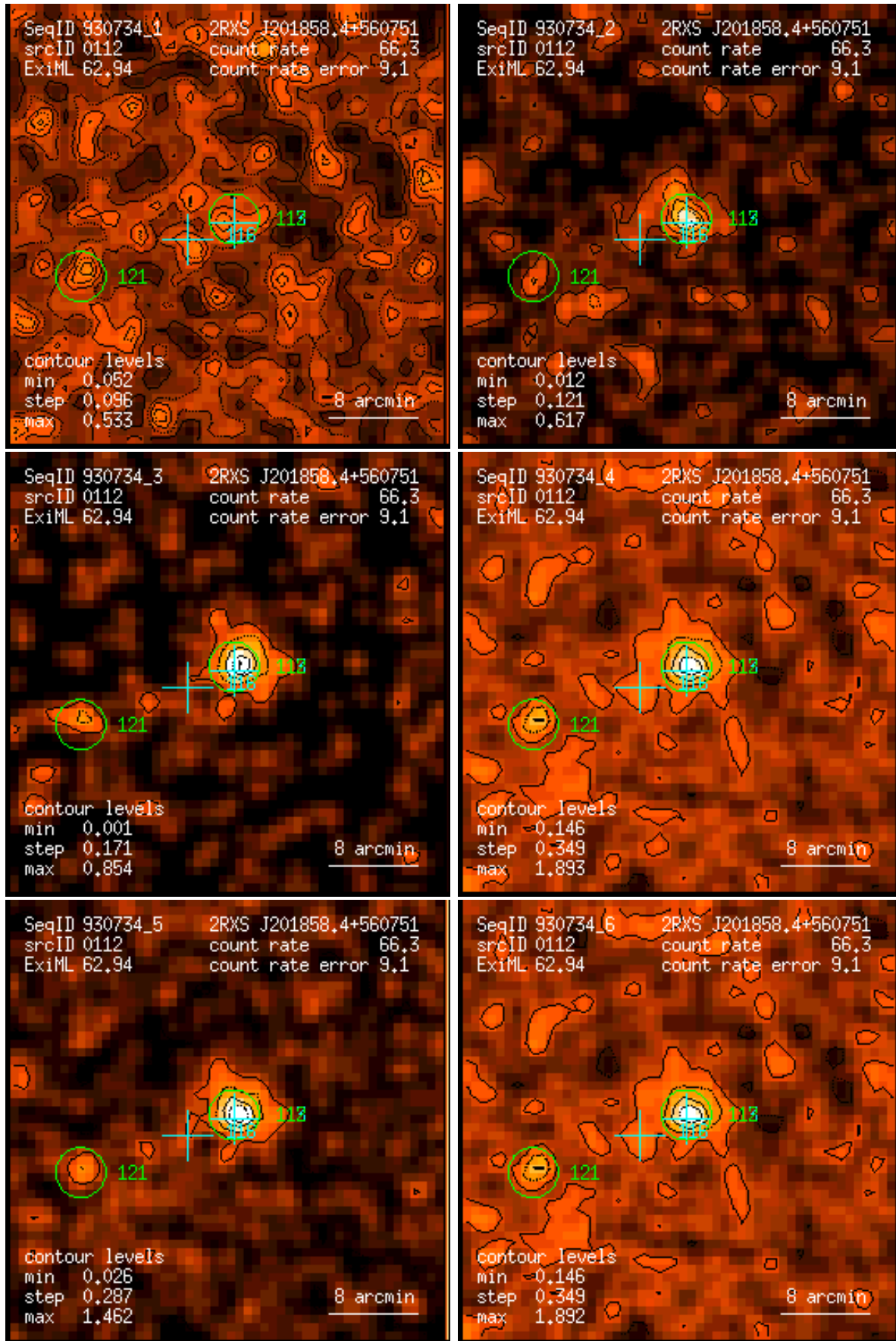
Figure 112: RASS 930734: detection 0112: band rate images, Gaussian filter: (1) PSPC channels 11 – 41, (2) 52 – 90, (3) 91 – 201, (4) 11 – 235, (5) 52 – 201, (6) 11 – 201. Broad band rates in counts/ks. Band rate contour levels in counts/ks/arcmin 2 .
