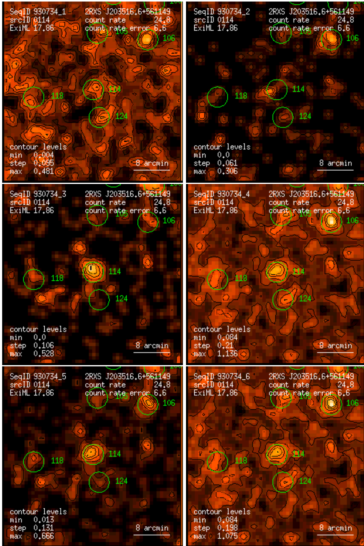
Figure 114: RASS 930734: detection 0114: band rate images, Gaussian filter: (1) PSPC channels 11 – 41, (2) 52 – 90, (3) 91 – 201, (4) 11 – 235, (5) 52 – 201, (6) 11 – 201. Broad band rates in counts/ks. Band rate contour levels in counts/ks/arcmin 2 .
