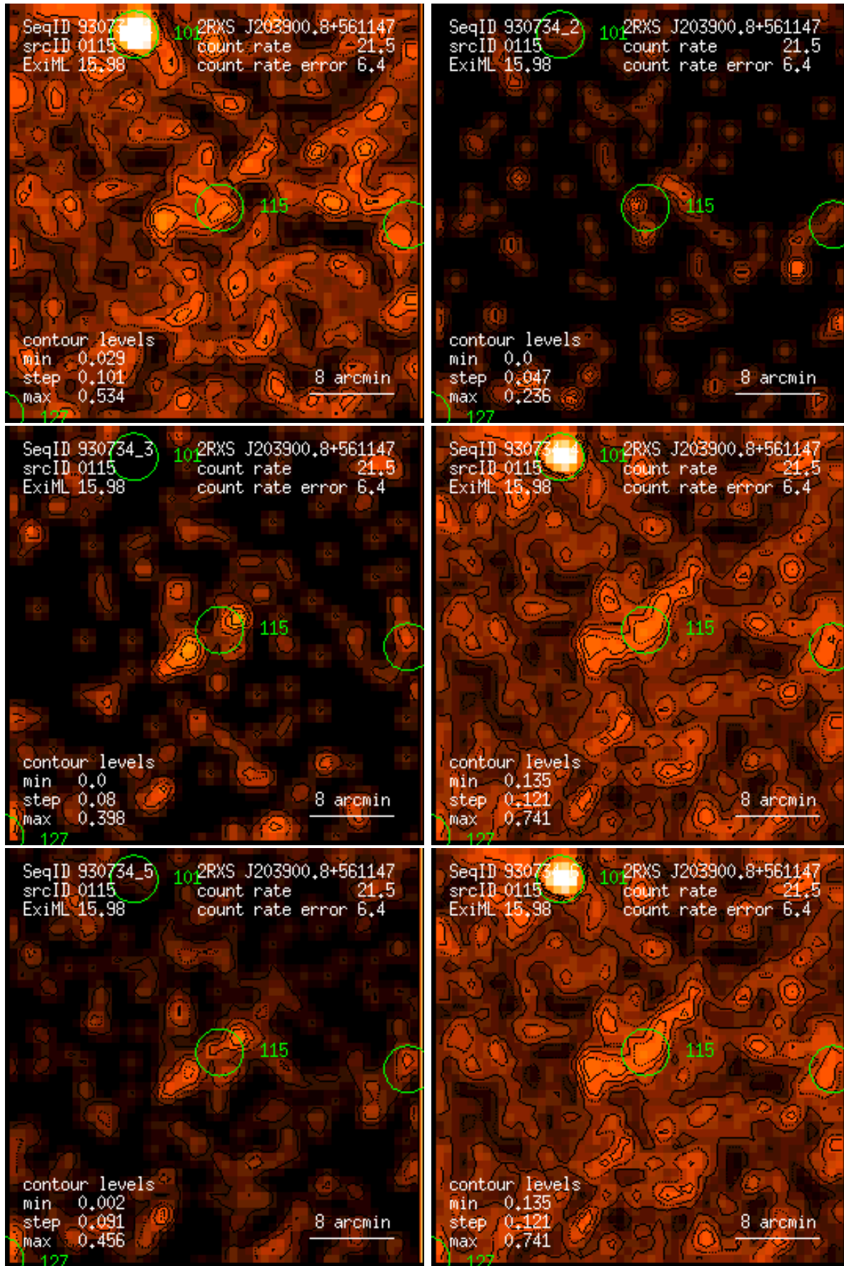
Figure 115: RASS 930734: detection 0115: band rate images, Gaussian filter: (1) PSPC channels 11 – 41, (2) 52 – 90, (3) 91 – 201, (4) 11 – 235, (5) 52 – 201, (6) 11 – 201. Broad band rates in counts/ks. Band rate contour levels in counts/ks/arcmin 2 .
