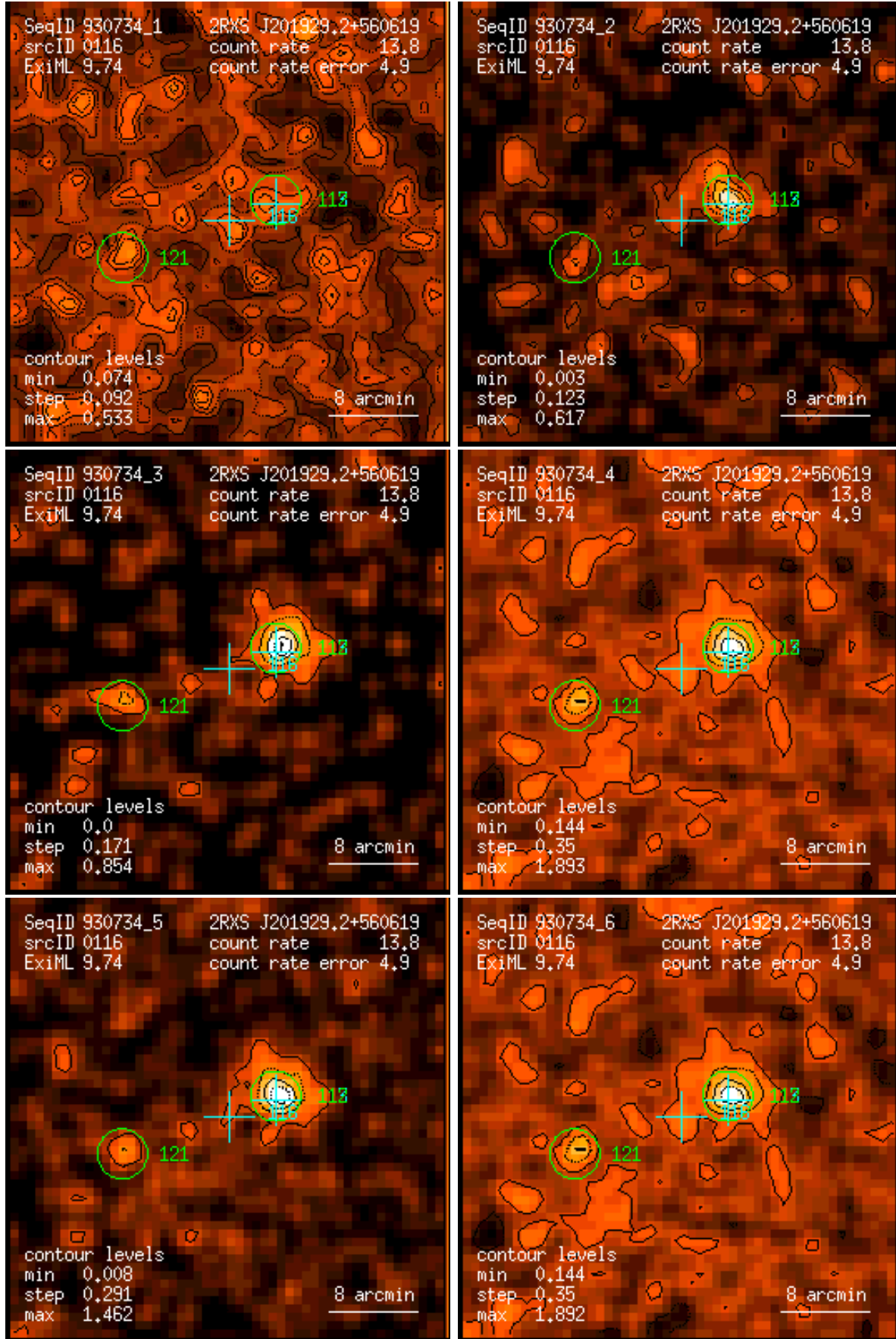
Figure 116: RASS 930734: detection 0116: band rate images, Gaussian filter: (1) PSPC channels 11 – 41, (2) 52 – 90, (3) 91 – 201, (4) 11 – 235, (5) 52 – 201, (6) 11 – 201. Broad band rates in counts/ks. Band rate contour levels in counts/ks/arcmin 2 .
