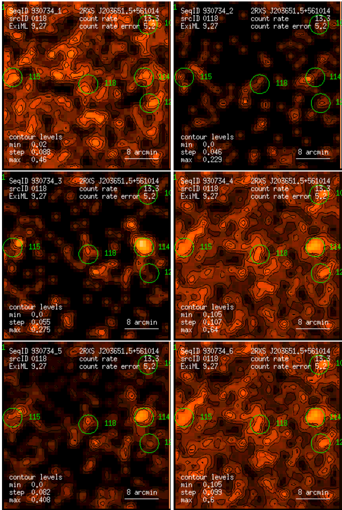
Figure 118: RASS 930734: detection 0118: band rate images, Gaussian filter: (1) PSPC channels 11 – 41, (2) 52 – 90, (3) 91 – 201, (4) 11 – 235, (5) 52 – 201, (6) 11 – 201. Broad band rates in counts/ks. Band rate contour levels in counts/ks/arcmin 2 .
