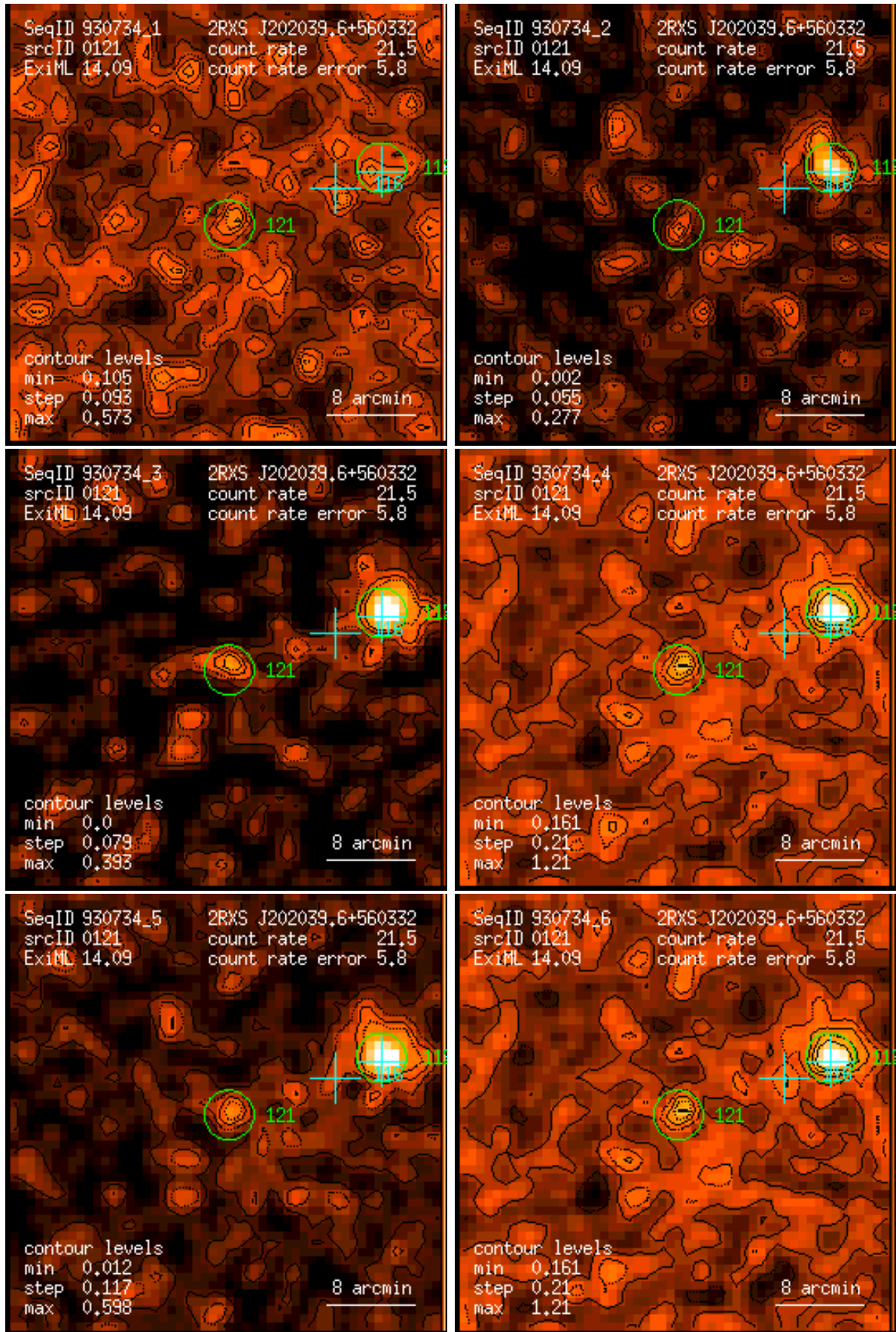
Figure 121: RASS 930734: detection 0121: band rate images, Gaussian filter: (1) PSPC channels 11 – 41, (2) 52 – 90, (3) 91 – 201, (4) 11 – 235, (5) 52 – 201, (6) 11 – 201. Broad band rates in counts/ks. Band rate contour levels in counts/ks/arcmin 2 .
