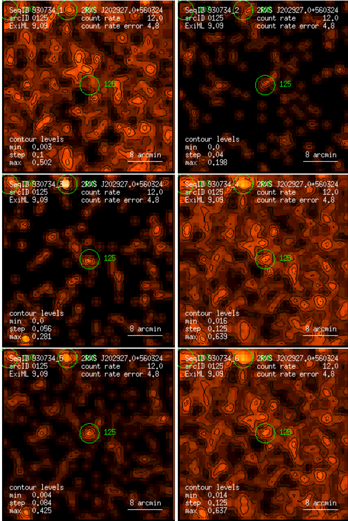
Figure 125: RASS 930734: detection 0125: band rate images, Gaussian filter: (1) PSPC channels 11 – 41, (2) 52 – 90, (3) 91 – 201, (4) 11 – 235, (5) 52 – 201, (6) 11 – 201. Broad band rates in counts/ks. Band rate contour levels in counts/ks/arcmin 2 .
