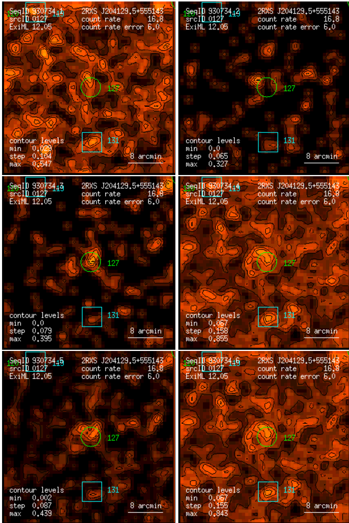
Figure 127: RASS 930734: detection 0127: band rate images, Gaussian filter: (1) PSPC channels 11 – 41, (2) 52 – 90, (3) 91 – 201, (4) 11 – 235, (5) 52 – 201, (6) 11 – 201. Broad band rates in counts/ks. Band rate contour levels in counts/ks/arcmin 2 .
