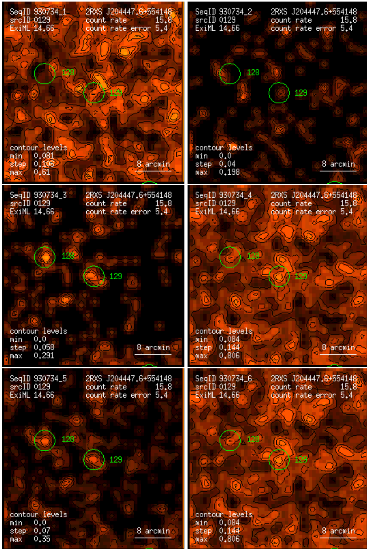
Figure 129: RASS 930734: detection 0129: band rate images, Gaussian filter: (1) PSPC channels 11 – 41, (2) 52 – 90, (3) 91 – 201, (4) 11 – 235, (5) 52 – 201, (6) 11 – 201. Broad band rates in counts/ks. Band rate contour levels in counts/ks/arcmin 2 .
