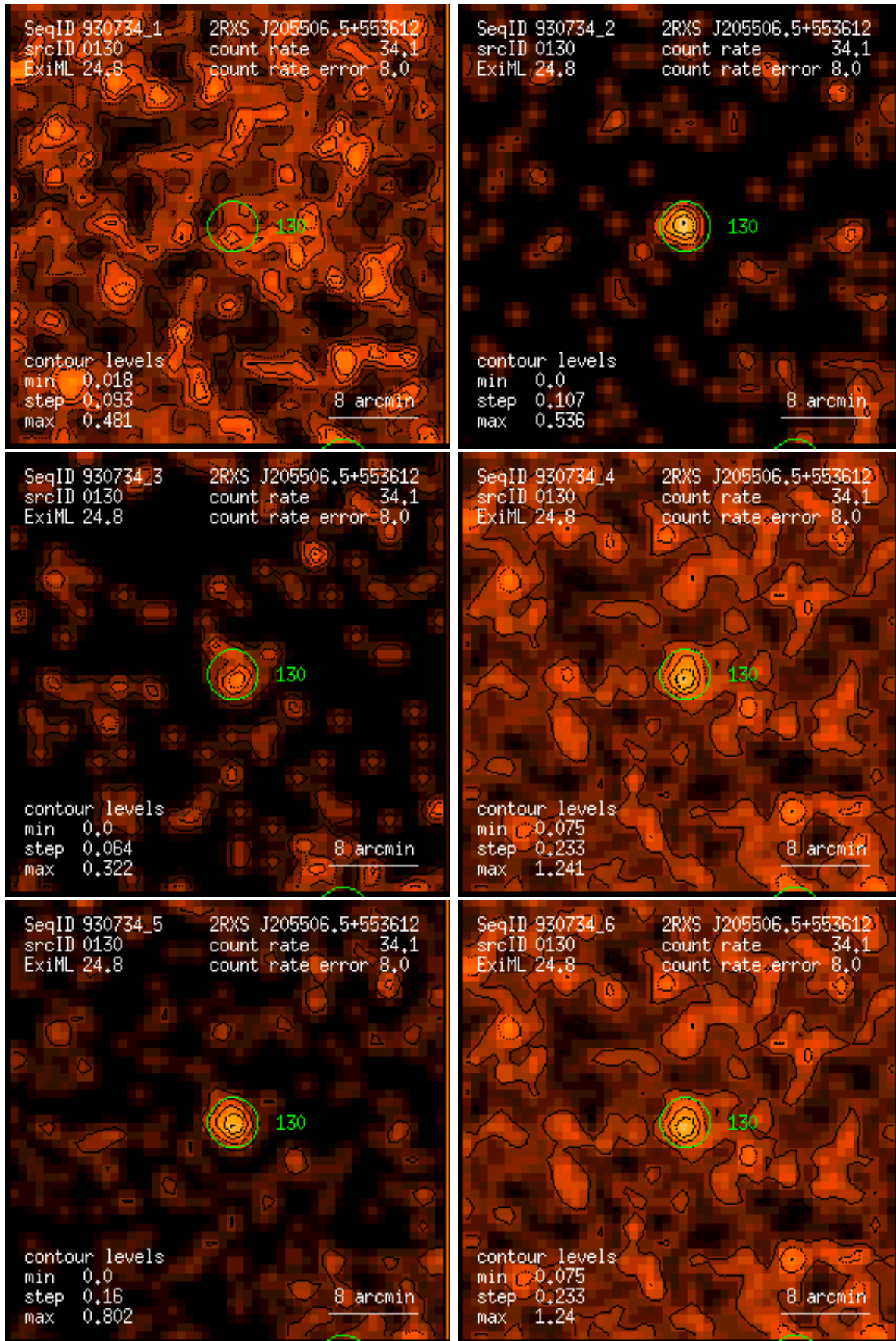
Figure 130: RASS 930734: detection 0130: band rate images, Gaussian filter: (1) PSPC channels 11 – 41, (2) 52 – 90, (3) 91 – 201, (4) 11 – 235, (5) 52 – 201, (6) 11 – 201. Broad band rates in counts/ks. Band rate contour levels in counts/ks/arcmin 2 .
