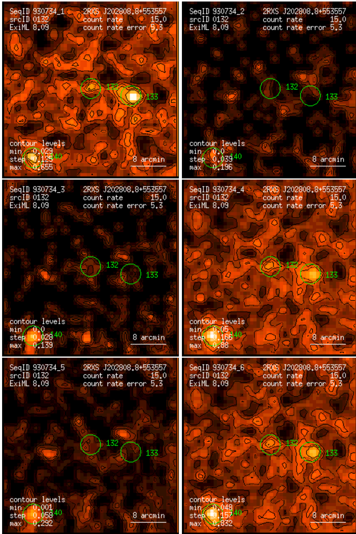
Figure 132: RASS 930734: detection 0132: band rate images, Gaussian filter: (1) PSPC channels 11 – 41, (2) 52 – 90, (3) 91 – 201, (4) 11 – 235, (5) 52 – 201, (6) 11 – 201. Broad band rates in counts/ks. Band rate contour levels in counts/ks/arcmin 2 .
