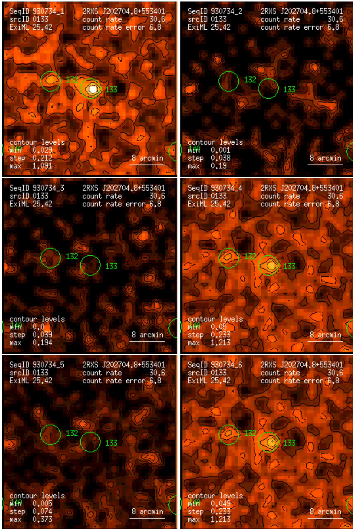
Figure 133: RASS 930734: detection 0133: band rate images, Gaussian filter: (1) PSPC channels 11 – 41, (2) 52 – 90, (3) 91 – 201, (4) 11 – 235, (5) 52 – 201, (6) 11 – 201. Broad band rates in counts/ks. Band rate contour levels in counts/ks/arcmin 2 .
