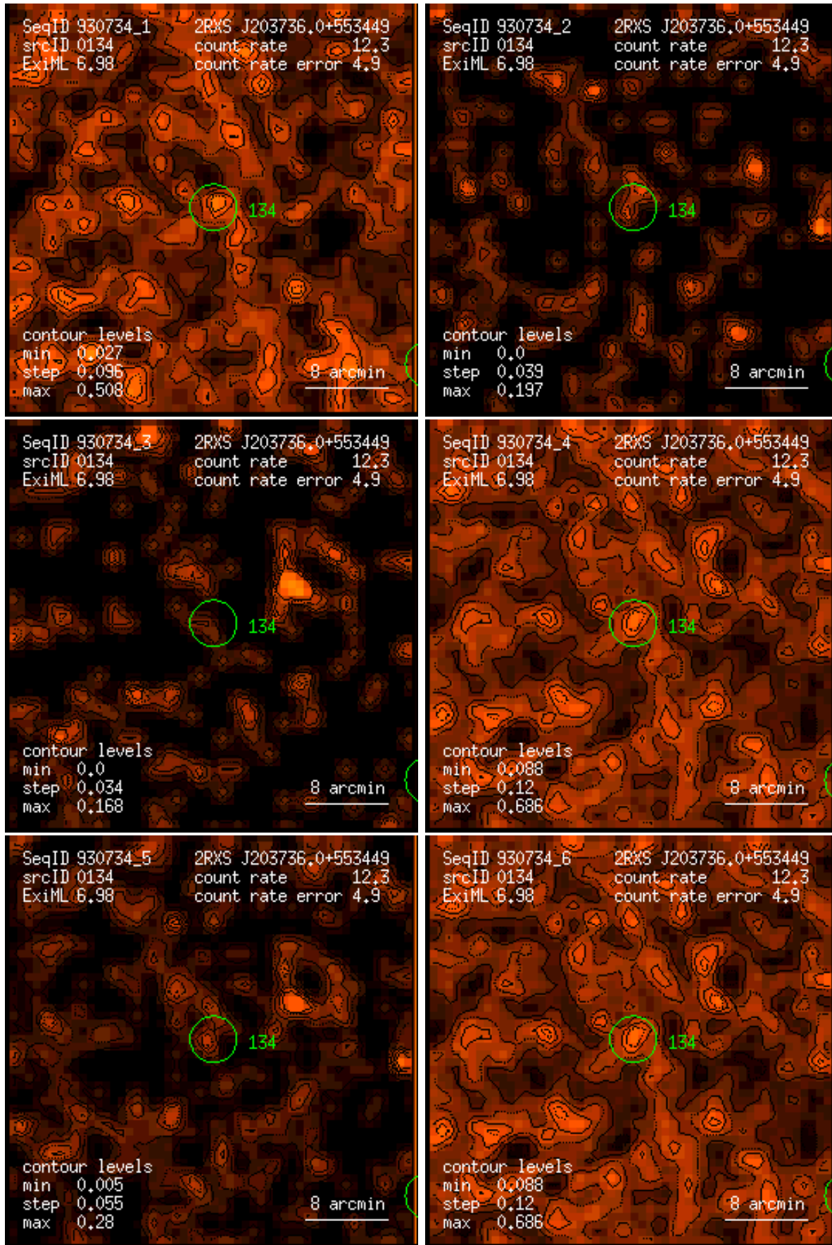
Figure 134: RASS 930734: detection 0134: band rate images, Gaussian filter: (1) PSPC channels 11 – 41, (2) 52 – 90, (3) 91 – 201, (4) 11 – 235, (5) 52 – 201, (6) 11 – 201. Broad band rates in counts/ks. Band rate contour levels in counts/ks/arcmin 2 .
