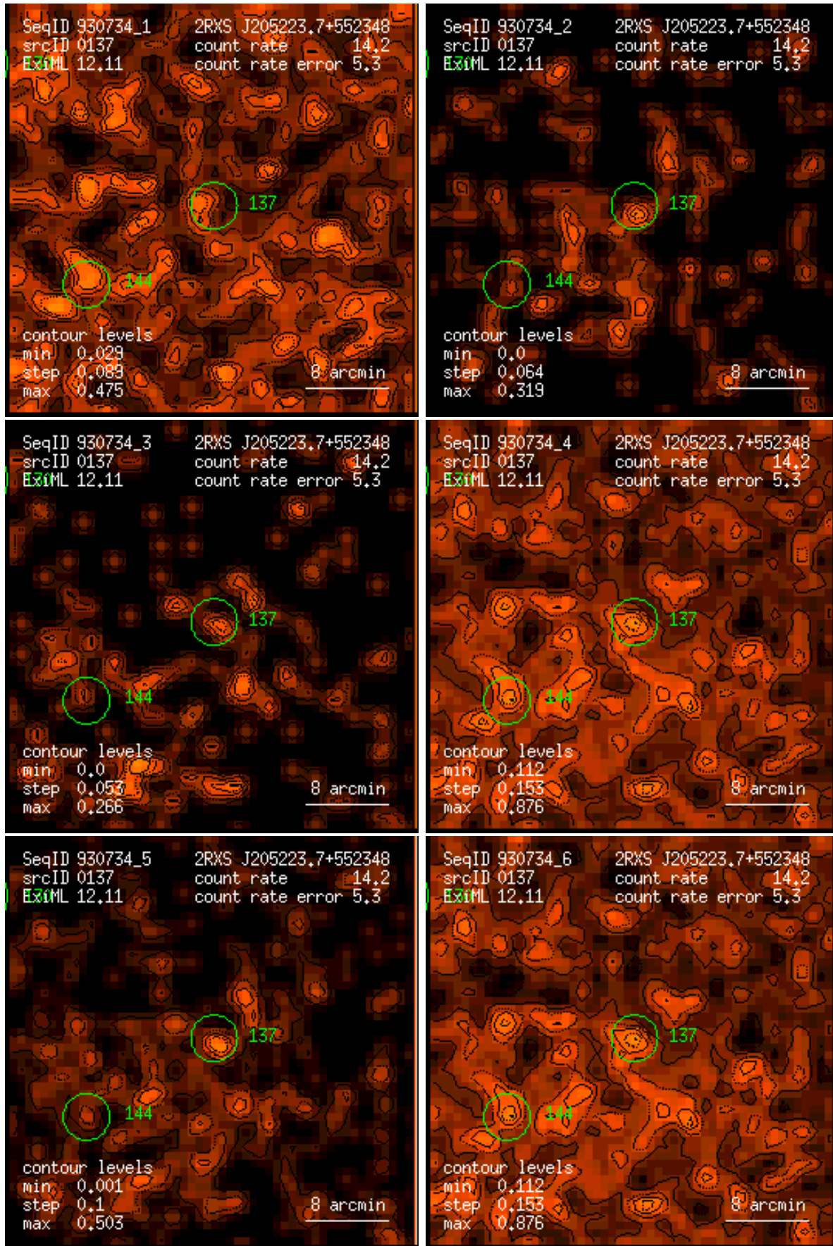
Figure 137: RASS 930734: detection 0137: band rate images, Gaussian filter: (1) PSPC channels 11 – 41, (2) 52 – 90, (3) 91 – 201, (4) 11 – 235, (5) 52 – 201, (6) 11 – 201. Broad band rates in counts/ks. Band rate contour levels in counts/ks/arcmin 2 .
