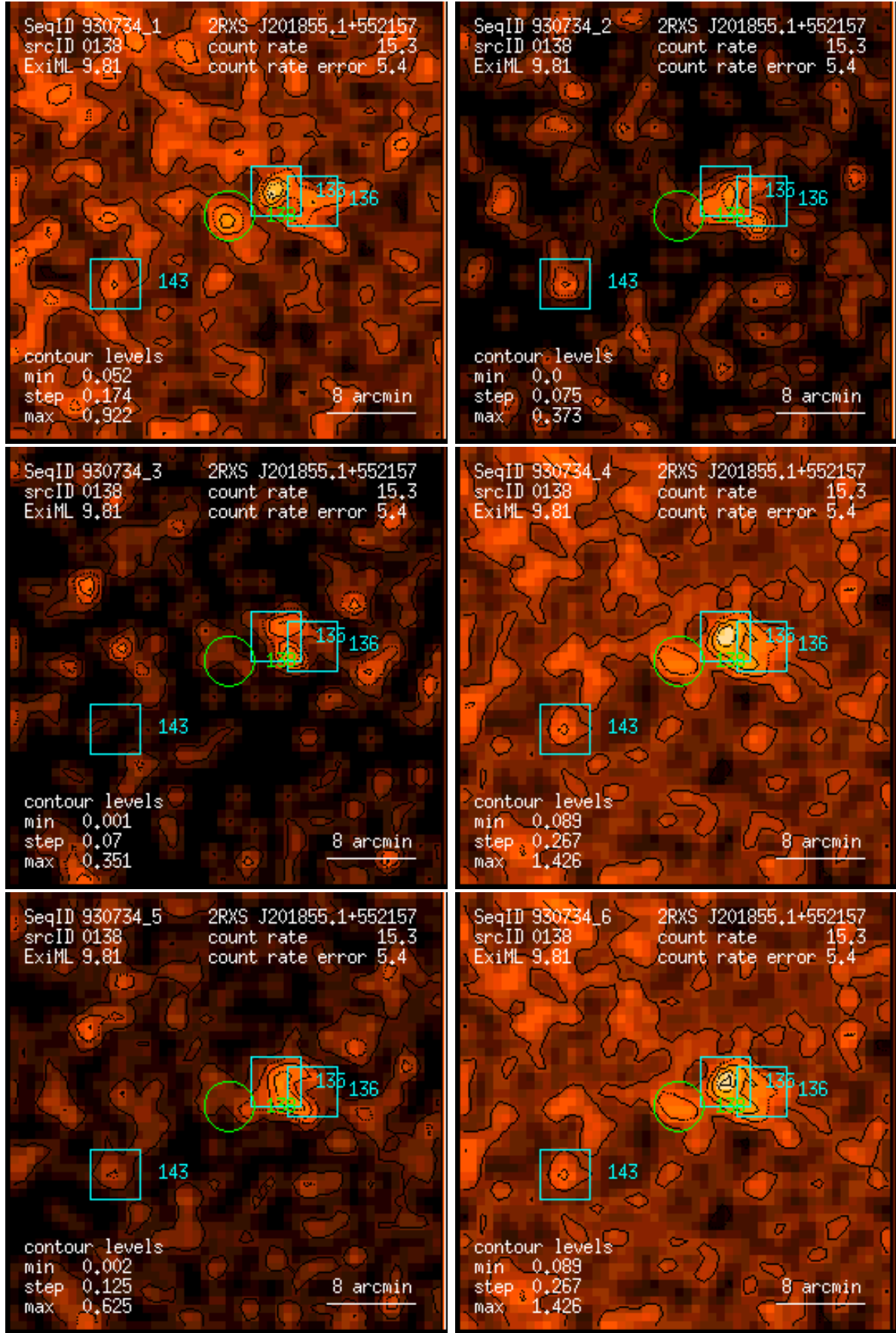
Figure 138: RASS 930734: detection 0138: band rate images, Gaussian filter: (1) PSPC channels 11 – 41, (2) 52 – 90, (3) 91 – 201, (4) 11 – 235, (5) 52 – 201, (6) 11 – 201. Broad band rates in counts/ks. Band rate contour levels in counts/ks/arcmin 2 .
