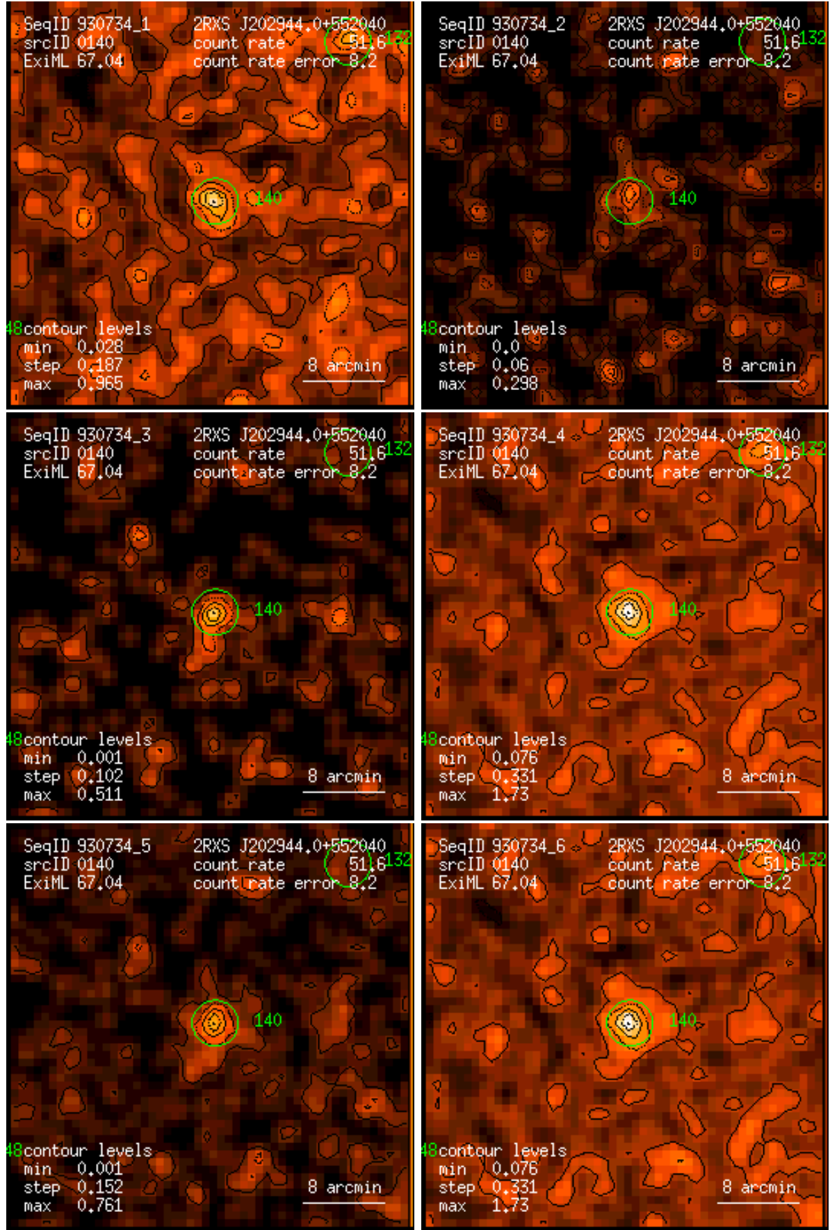
Figure 140: RASS 930734: detection 0140: band rate images, Gaussian filter: (1) PSPC channels 11 – 41, (2) 52 – 90, (3) 91 – 201, (4) 11 – 235, (5) 52 – 201, (6) 11 – 201. Broad band rates in counts/ks. Band rate contour levels in counts/ks/arcmin 2 .
