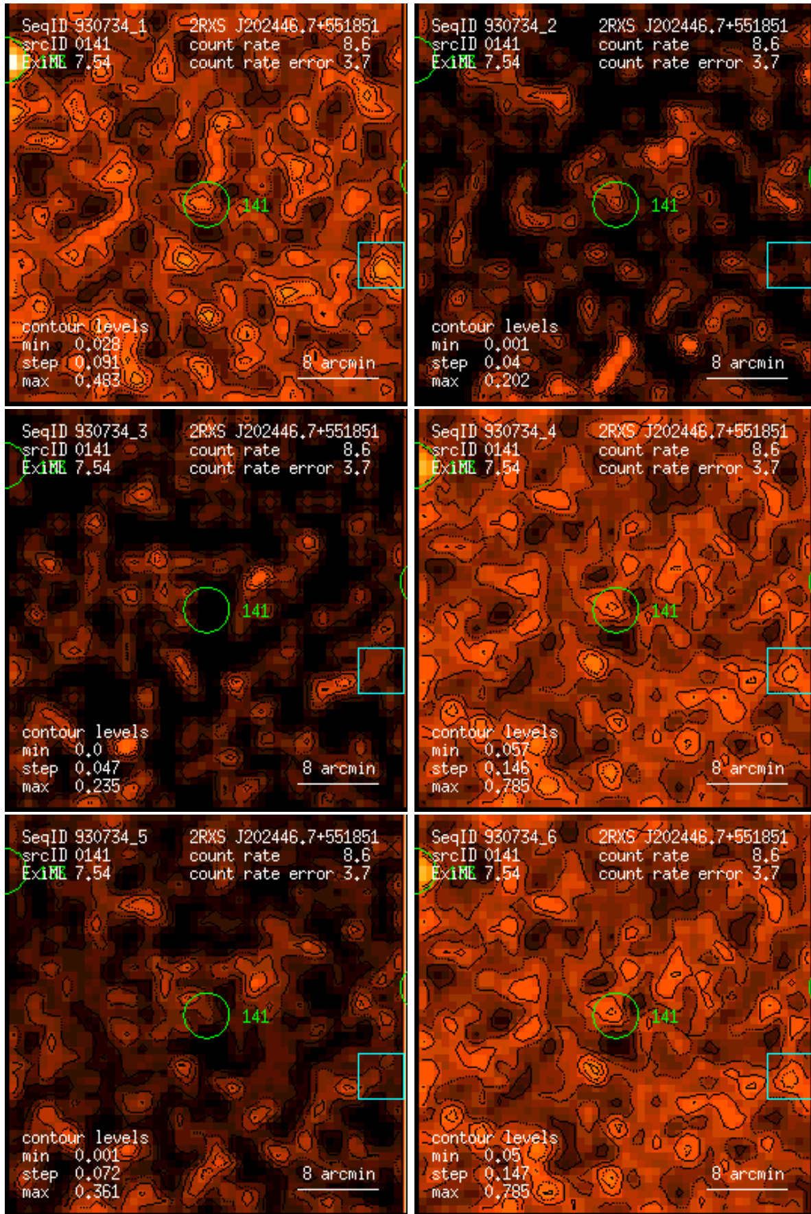
Figure 141: RASS 930734: detection 0141: band rate images, Gaussian filter: (1) PSPC channels 11 – 41, (2) 52 – 90, (3) 91 – 201, (4) 11 – 235, (5) 52 – 201, (6) 11 – 201. Broad band rates in counts/ks. Band rate contour levels in counts/ks/arcmin 2 .
