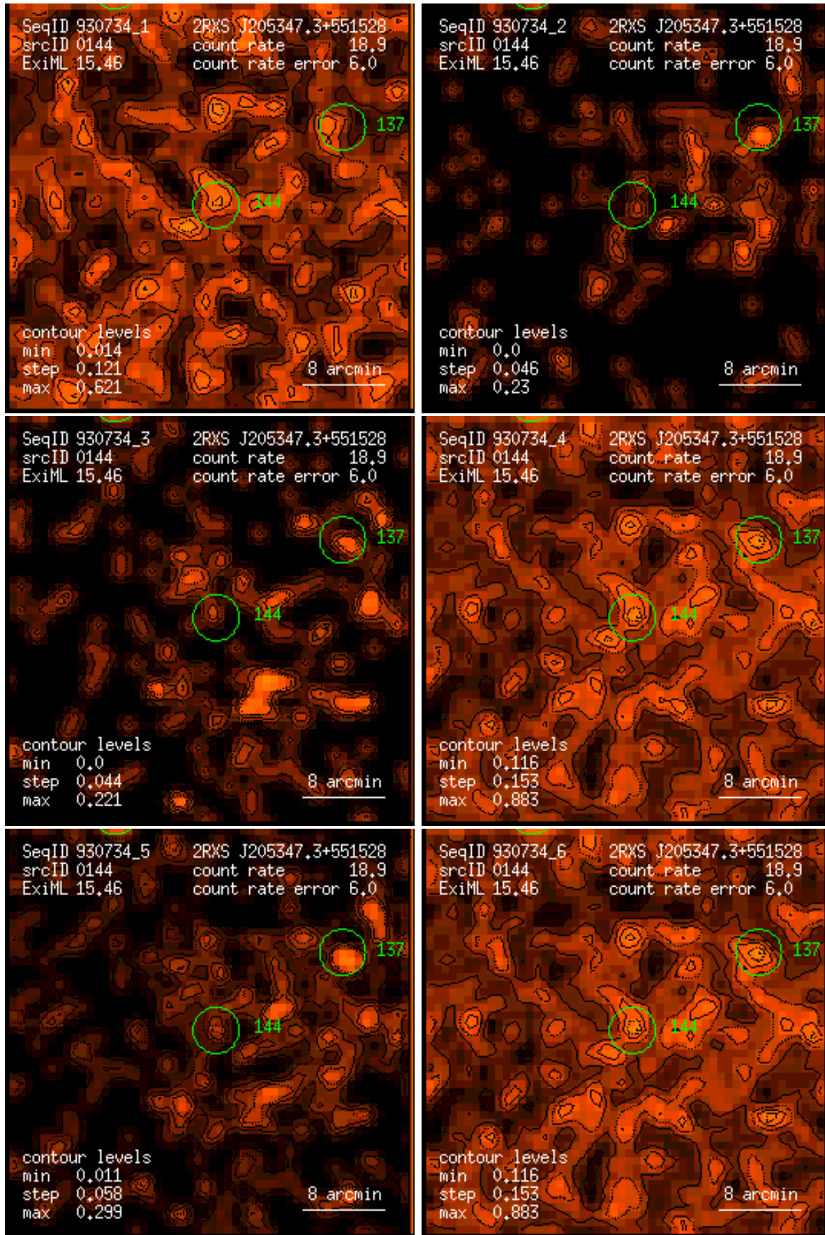
Figure 144: RASS 930734: detection 0144: band rate images, Gaussian filter: (1) PSPC channels 11 – 41, (2) 52 – 90, (3) 91 – 201, (4) 11 – 235, (5) 52 – 201, (6) 11 – 201. Broad band rates in counts/ks. Band rate contour levels in counts/ks/arcmin 2 .
