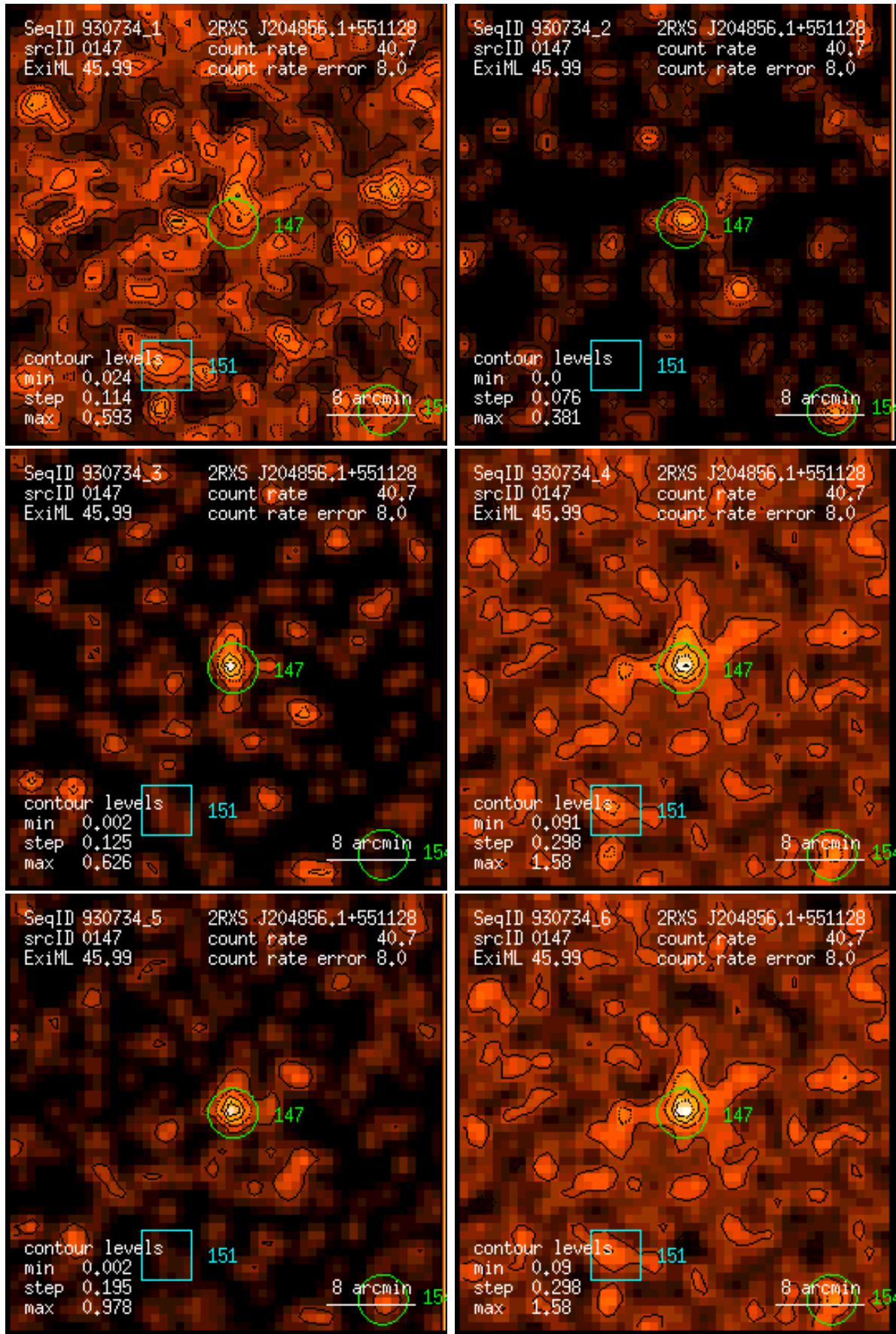
Figure 147: RASS 930734: detection 0147: band rate images, Gaussian filter: (1) PSPC channels 11 – 41, (2) 52 – 90, (3) 91 – 201, (4) 11 – 235, (5) 52 – 201, (6) 11 – 201. Broad band rates in counts/ks. Band rate contour levels in counts/ks/arcmin 2 .
