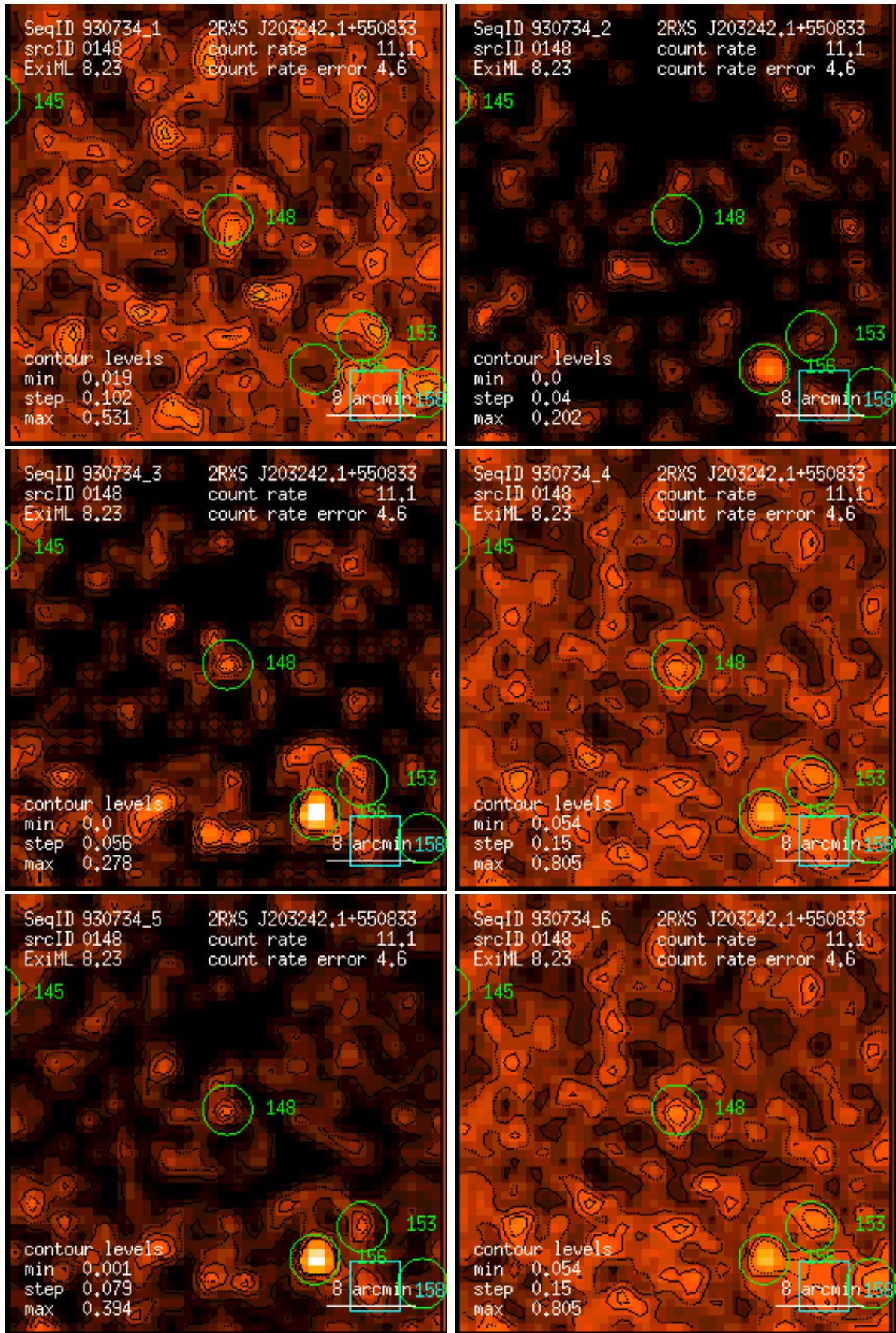
Figure 148: RASS 930734: detection 0148: band rate images, Gaussian filter: (1) PSPC channels 11 – 41, (2) 52 – 90, (3) 91 – 201, (4) 11 – 235, (5) 52 – 201, (6) 11 – 201. Broad band rates in counts/ks. Band rate contour levels in counts/ks/arcmin 2 .
