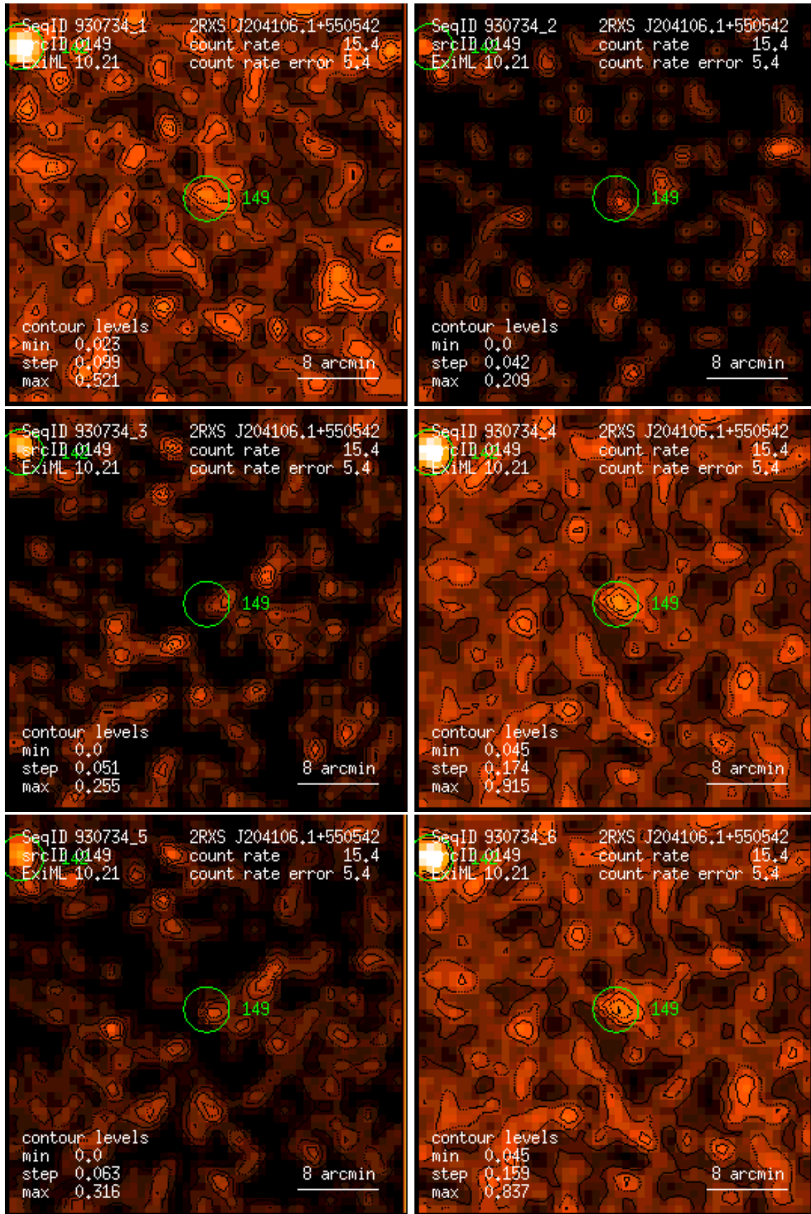
Figure 149: RASS 930734: detection 0149: band rate images, Gaussian filter: (1) PSPC channels 11 – 41, (2) 52 – 90, (3) 91 – 201, (4) 11 – 235, (5) 52 – 201, (6) 11 – 201. Broad band rates in counts/ks. Band rate contour levels in counts/ks/arcmin 2 .
