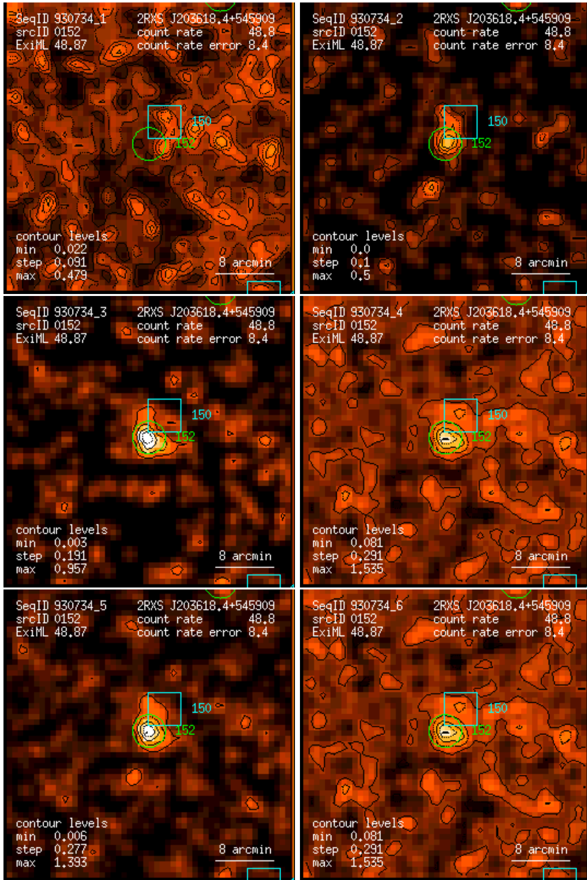
Figure 152: RASS 930734: detection 0152: band rate images, Gaussian filter: (1) PSPC channels 11 – 41, (2) 52 – 90, (3) 91 – 201, (4) 11 – 235, (5) 52 – 201, (6) 11 – 201. Broad band rates in counts/ks. Band rate contour levels in counts/ks/arcmin 2 .
