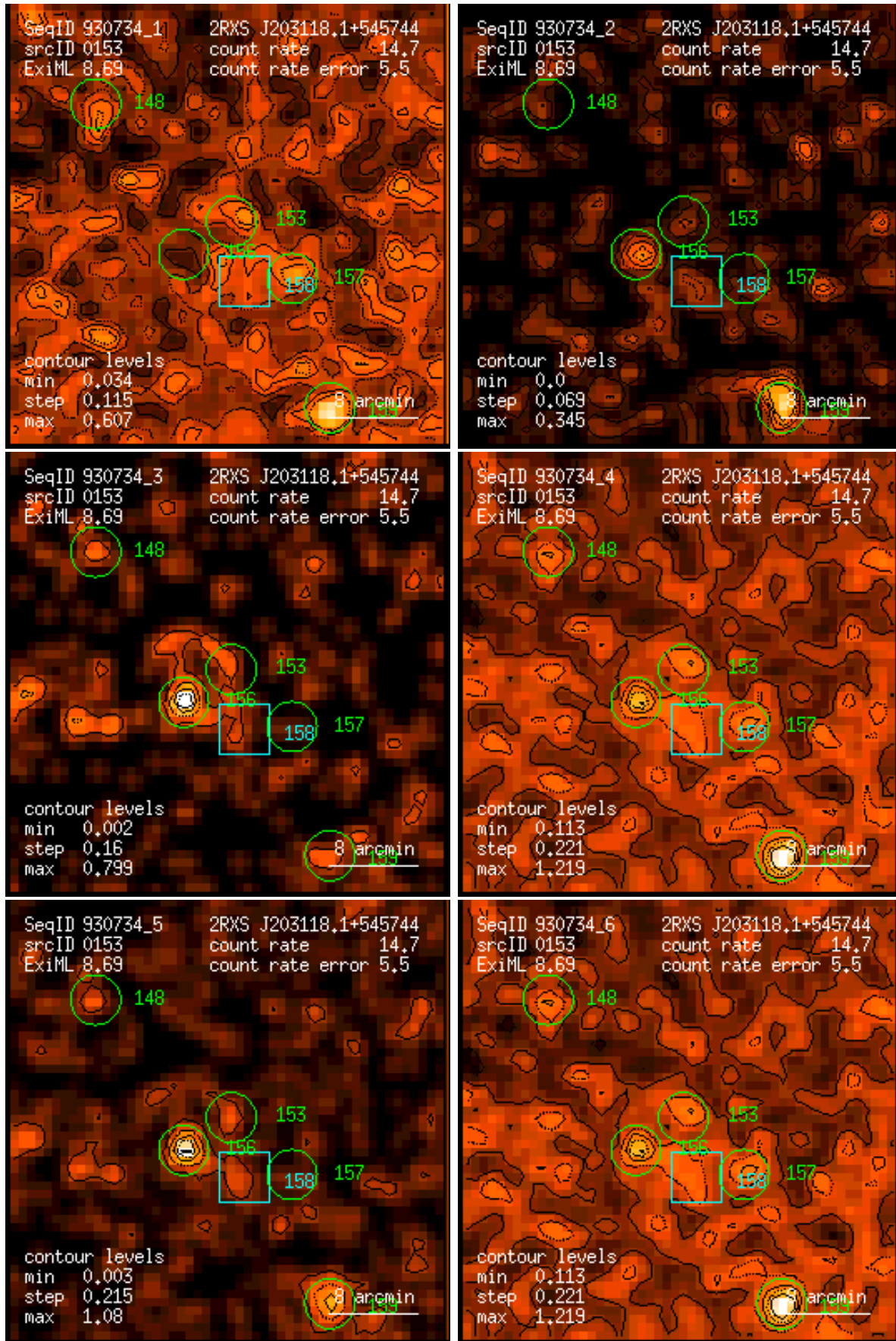
Figure 153: RASS 930734: detection 0153: band rate images, Gaussian filter: (1) PSPC channels 11 – 41, (2) 52 – 90, (3) 91 – 201, (4) 11 – 235, (5) 52 – 201, (6) 11 – 201. Broad band rates in counts/ks. Band rate contour levels in counts/ks/arcmin 2 .
