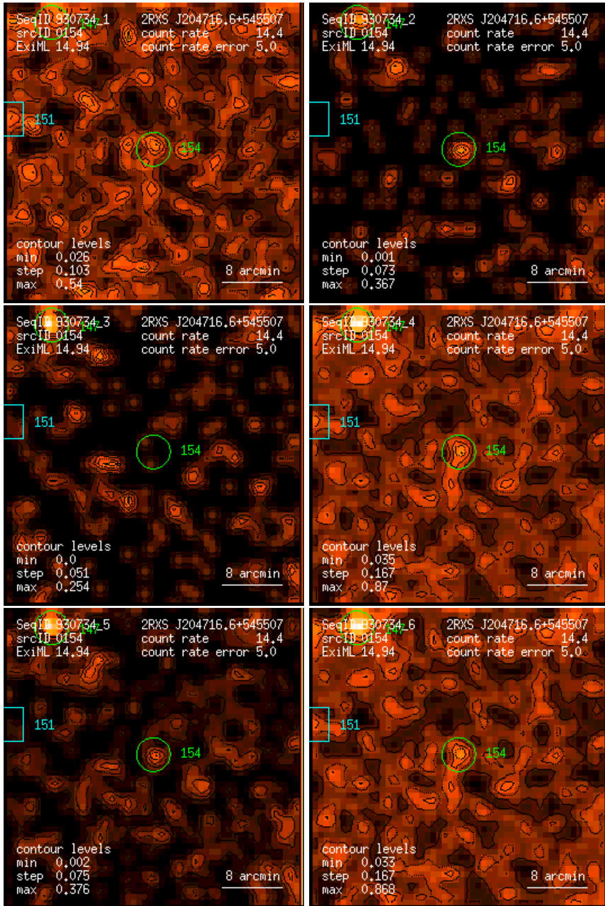
Figure 154: RASS 930734: detection 0154: band rate images, Gaussian filter: (1) PSPC channels 11 – 41, (2) 52 – 90, (3) 91 – 201, (4) 11 – 235, (5) 52 – 201, (6) 11 – 201. Broad band rates in counts/ks. Band rate contour levels in counts/ks/arcmin 2 .
