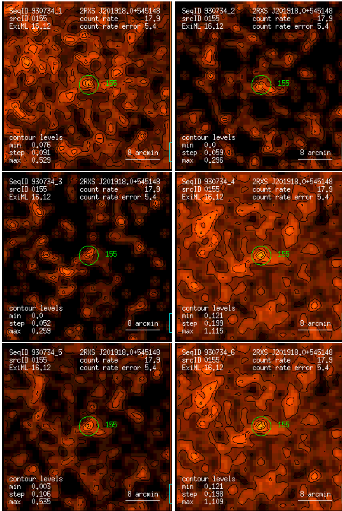
Figure 155: RASS 930734: detection 0155: band rate images, Gaussian filter: (1) PSPC channels 11 – 41, (2) 52 – 90, (3) 91 – 201, (4) 11 – 235, (5) 52 – 201, (6) 11 – 201. Broad band rates in counts/ks. Band rate contour levels in counts/ks/arcmin 2 .
