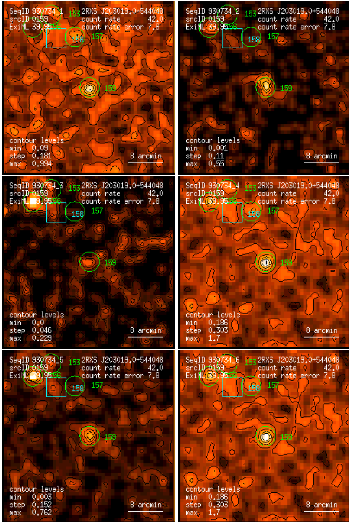
Figure 159: RASS 930734: detection 0159: band rate images, Gaussian filter: (1) PSPC channels 11 – 41, (2) 52 – 90, (3) 91 – 201, (4) 11 – 235, (5) 52 – 201, (6) 11 – 201. Broad band rates in counts/ks. Band rate contour levels in counts/ks/arcmin 2 .
