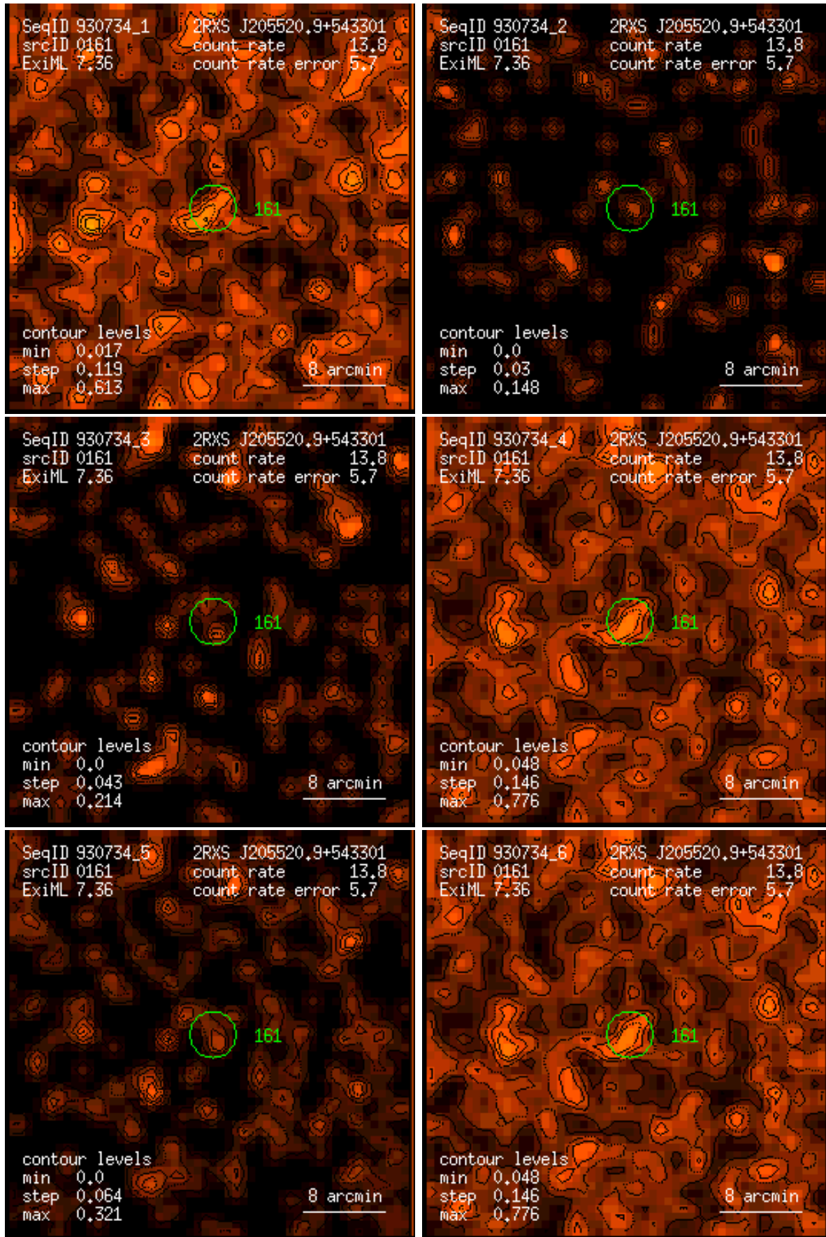
Figure 161: RASS 930734: detection 0161: band rate images, Gaussian filter: (1) PSPC channels 11 – 41, (2) 52 – 90, (3) 91 – 201, (4) 11 – 235, (5) 52 – 201, (6) 11 – 201. Broad band rates in counts/ks. Band rate contour levels in counts/ks/arcmin 2 .
