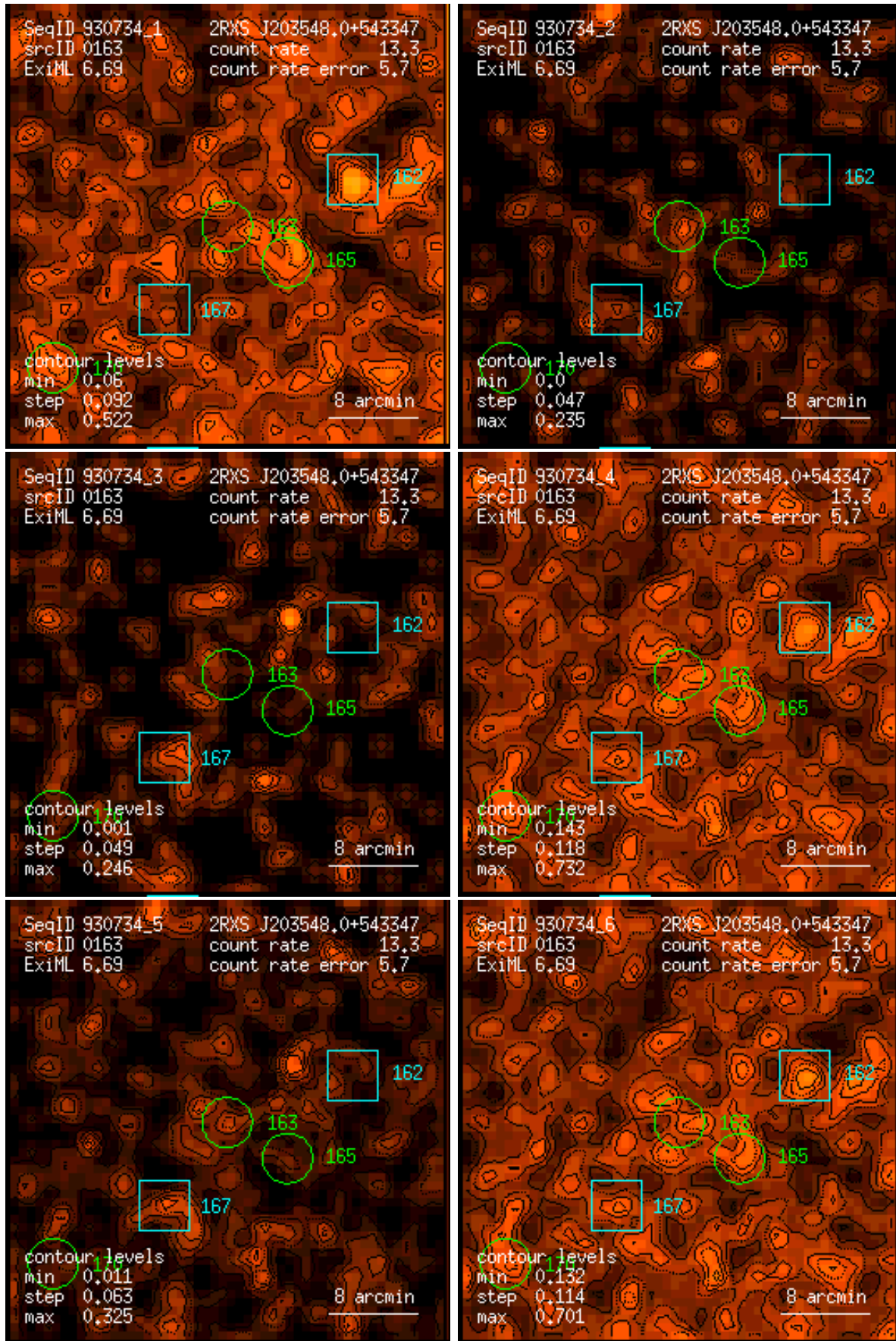
Figure 163: RASS 930734: detection 0163: band rate images, Gaussian filter: (1) PSPC channels 11 – 41, (2) 52 – 90, (3) 91 – 201, (4) 11 – 235, (5) 52 – 201, (6) 11 – 201. Broad band rates in counts/ks. Band rate contour levels in counts/ks/arcmin 2 .
